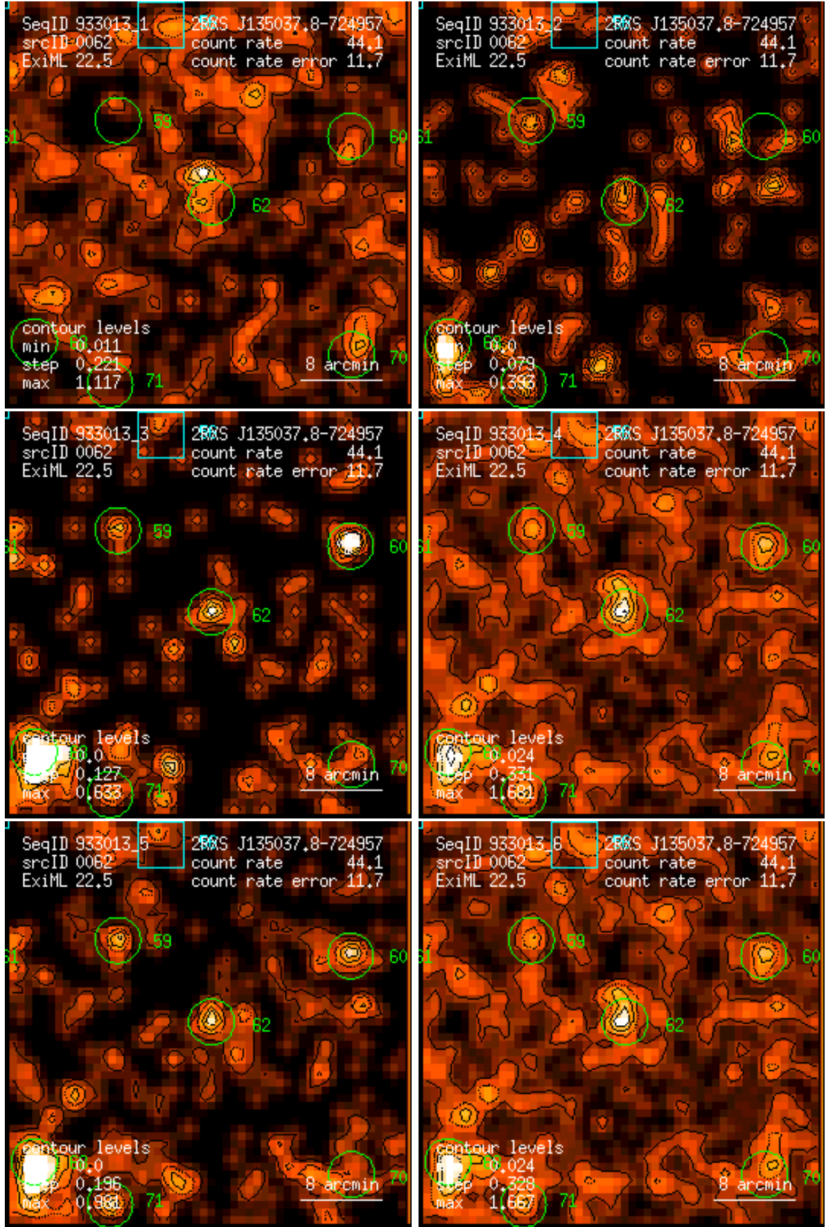
Figure 62: RASS 933013: detection 0062: band rate images, Gaussian filter: (1) PSPC channels 11 – 41, (2) 52 – 90, (3) 91 – 201, (4) 11 – 235, (5) 52 – 201, (6) 11 – 201. Broad band rates in counts/ks. Band rate contour levels in counts/ks/arcmin 2 .
