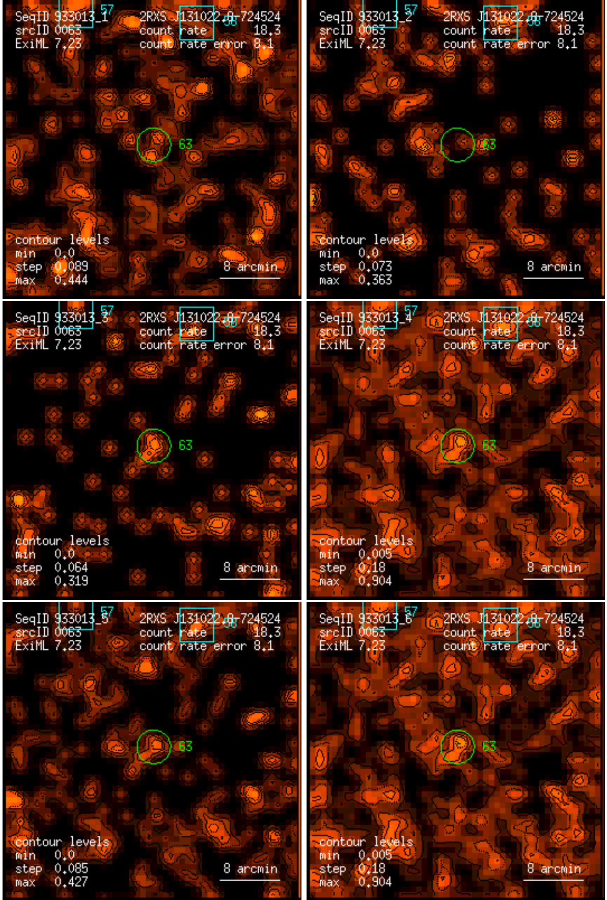
Figure 63: RASS 933013: detection 0063: band rate images, Gaussian filter: (1) PSPC channels 11 – 41, (2) 52 – 90, (3) 91 – 201, (4) 11 – 235, (5) 52 – 201, (6) 11 – 201. Broad band rates in counts/ks. Band rate contour levels in counts/ks/arcmin 2 .
