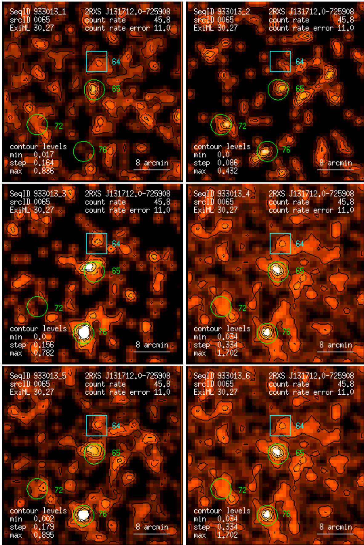
Figure 65: RASS 933013: detection 0065: band rate images, Gaussian filter: (1) PSPC channels 11 – 41, (2) 52 – 90, (3) 91 – 201, (4) 11 – 235, (5) 52 – 201, (6) 11 – 201. Broad band rates in counts/ks. Band rate contour levels in counts/ks/arcmin 2 .
