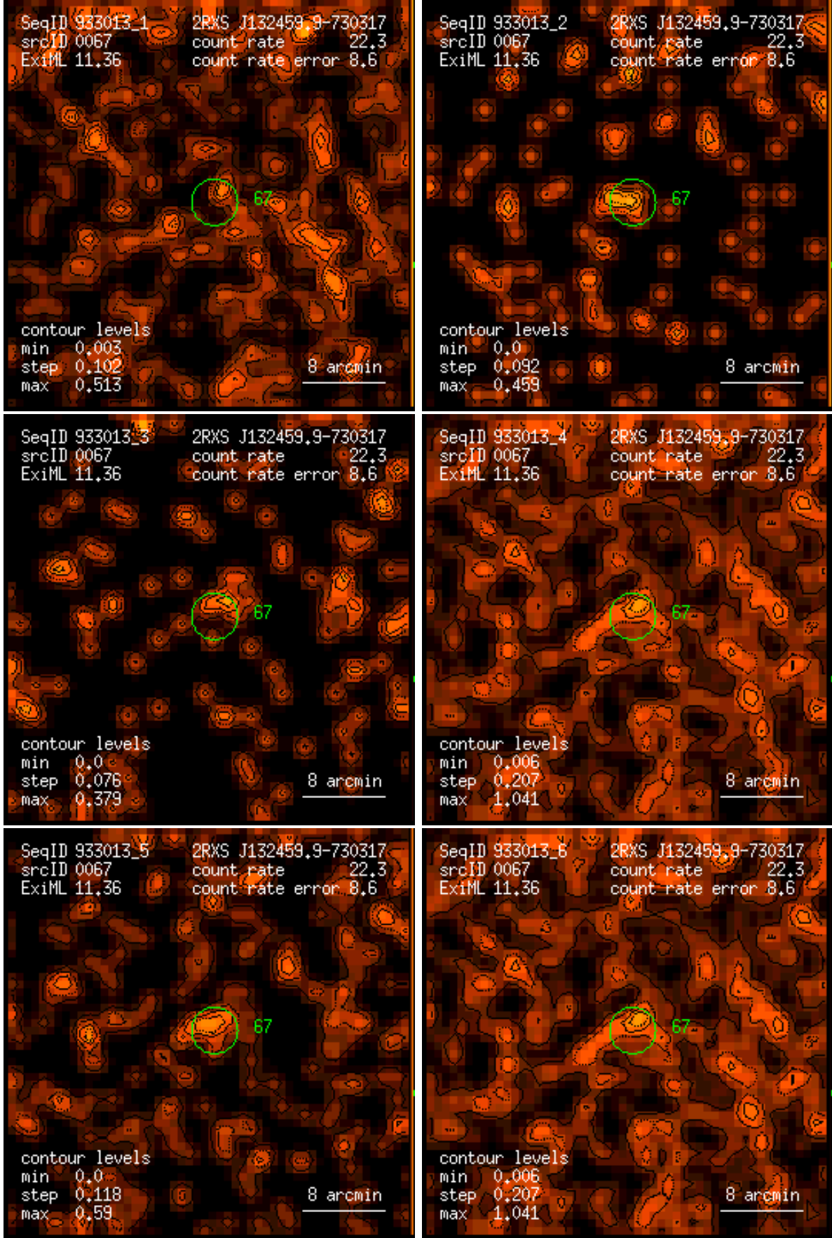
Figure 67: RASS 933013: detection 0067: band rate images, Gaussian filter: (1) PSPC channels 11 – 41, (2) 52 – 90, (3) 91 – 201, (4) 11 – 235, (5) 52 – 201, (6) 11 – 201. Broad band rates in counts/ks. Band rate contour levels in counts/ks/arcmin 2 .
