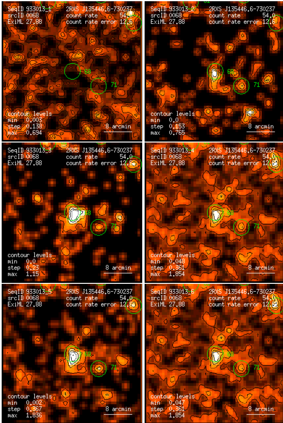
Figure 68: RASS 933013: detection 0068: band rate images, Gaussian filter: (1) PSPC channels 11 – 41, (2) 52 – 90, (3) 91 – 201, (4) 11 – 235, (5) 52 – 201, (6) 11 – 201. Broad band rates in counts/ks. Band rate contour levels in counts/ks/arcmin 2 .
