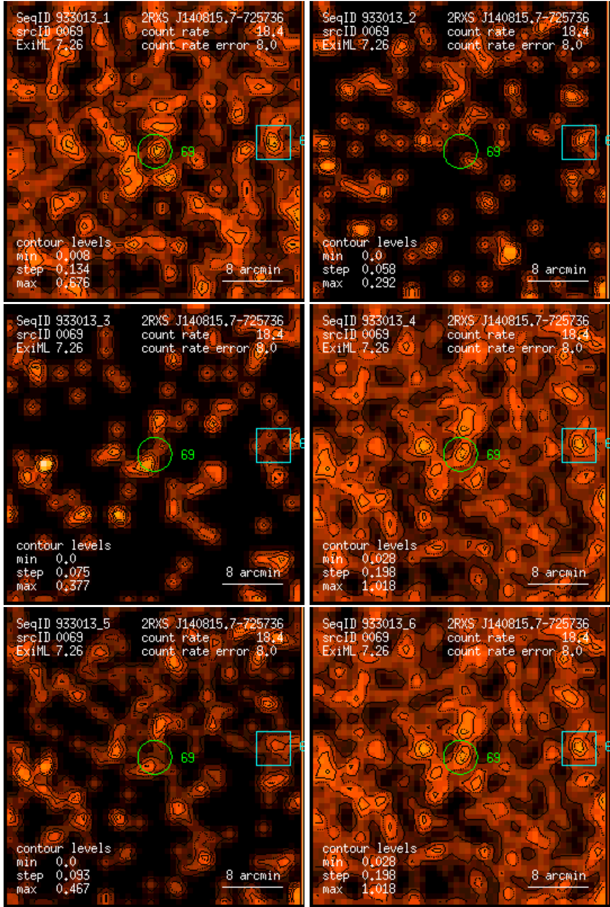
Figure 69: RASS 933013: detection 0069: band rate images, Gaussian filter: (1) PSPC channels 11 – 41, (2) 52 – 90, (3) 91 – 201, (4) 11 – 235, (5) 52 – 201, (6) 11 – 201. Broad band rates in counts/ks. Band rate contour levels in counts/ks/arcmin 2 .
