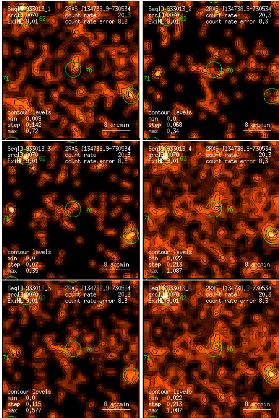
Figure 70: RASS 933013: detection 0070: band rate images, Gaussian filter: (1) PSPC channels 11 – 41, (2) 52 – 90, (3) 91 – 201, (4) 11 – 235, (5) 52 – 201, (6) 11 – 201. Broad band rates in counts/ks. Band rate contour levels in counts/ks/arcmin 2 .
