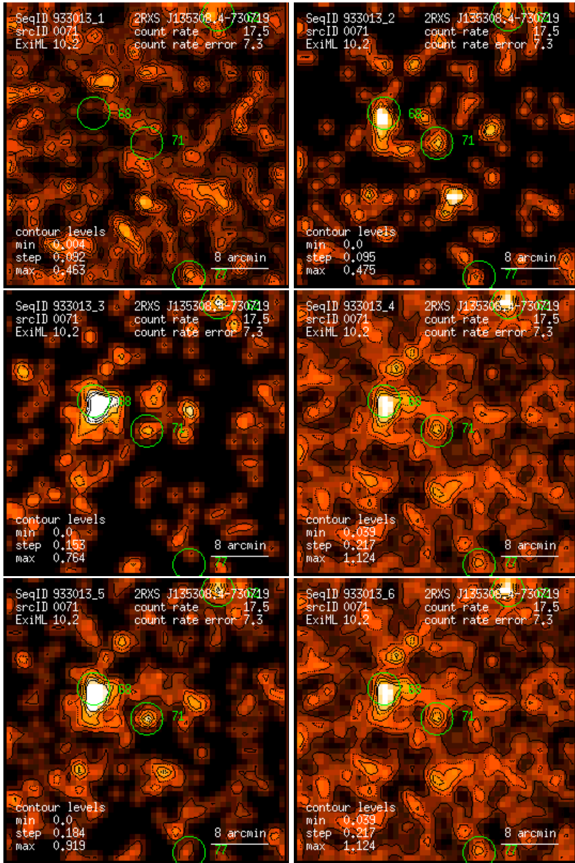
Figure 71: RASS 933013: detection 0071: band rate images, Gaussian filter: (1) PSPC channels 11 – 41, (2) 52 – 90, (3) 91 – 201, (4) 11 – 235, (5) 52 – 201, (6) 11 – 201. Broad band rates in counts/ks. Band rate contour levels in counts/ks/arcmin 2 .
