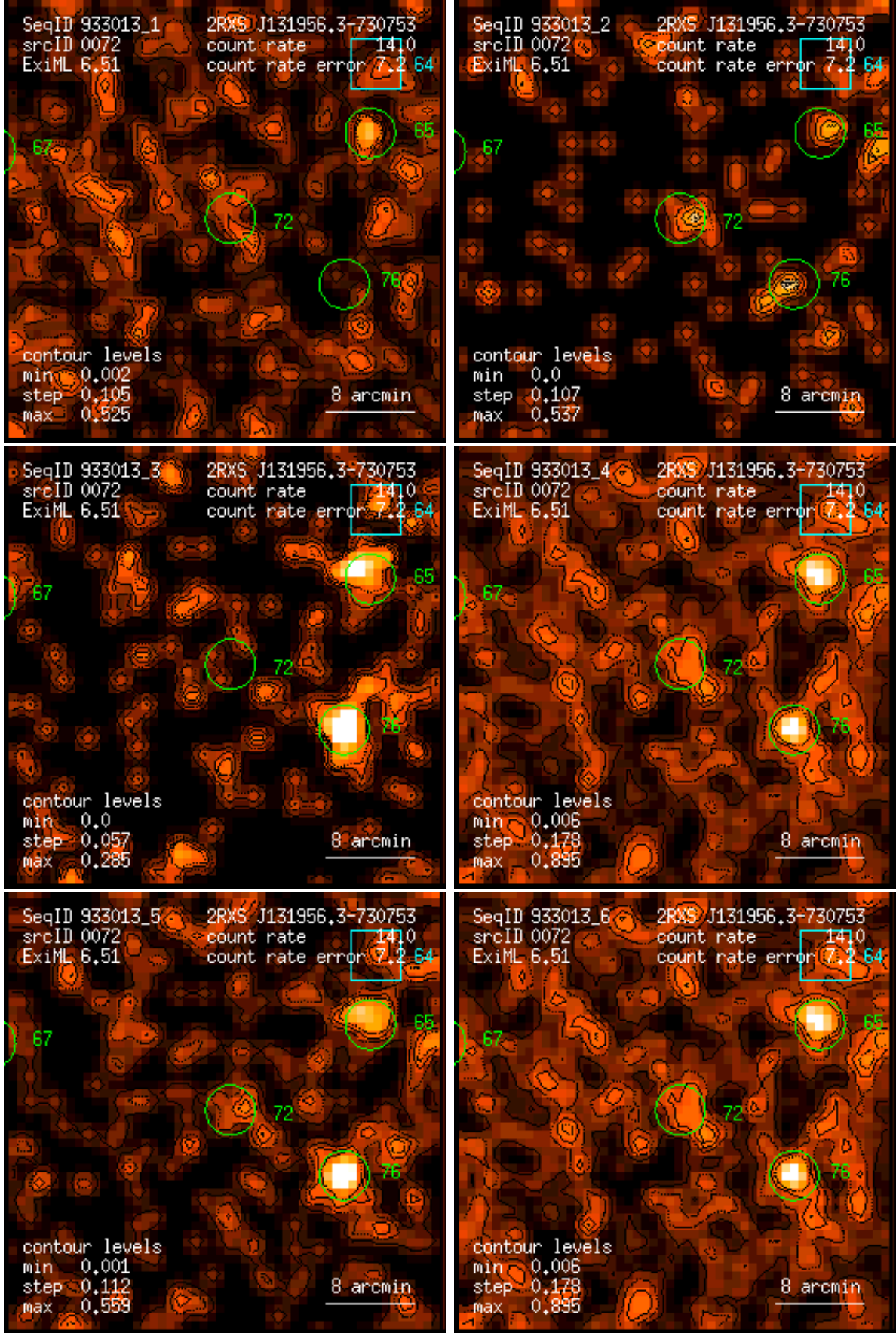
Figure 72: RASS 933013: detection 0072: band rate images, Gaussian filter: (1) PSPC channels 11 – 41, (2) 52 – 90, (3) 91 – 201, (4) 11 – 235, (5) 52 – 201, (6) 11 – 201. Broad band rates in counts/ks. Band rate contour levels in counts/ks/arcmin 2 .
