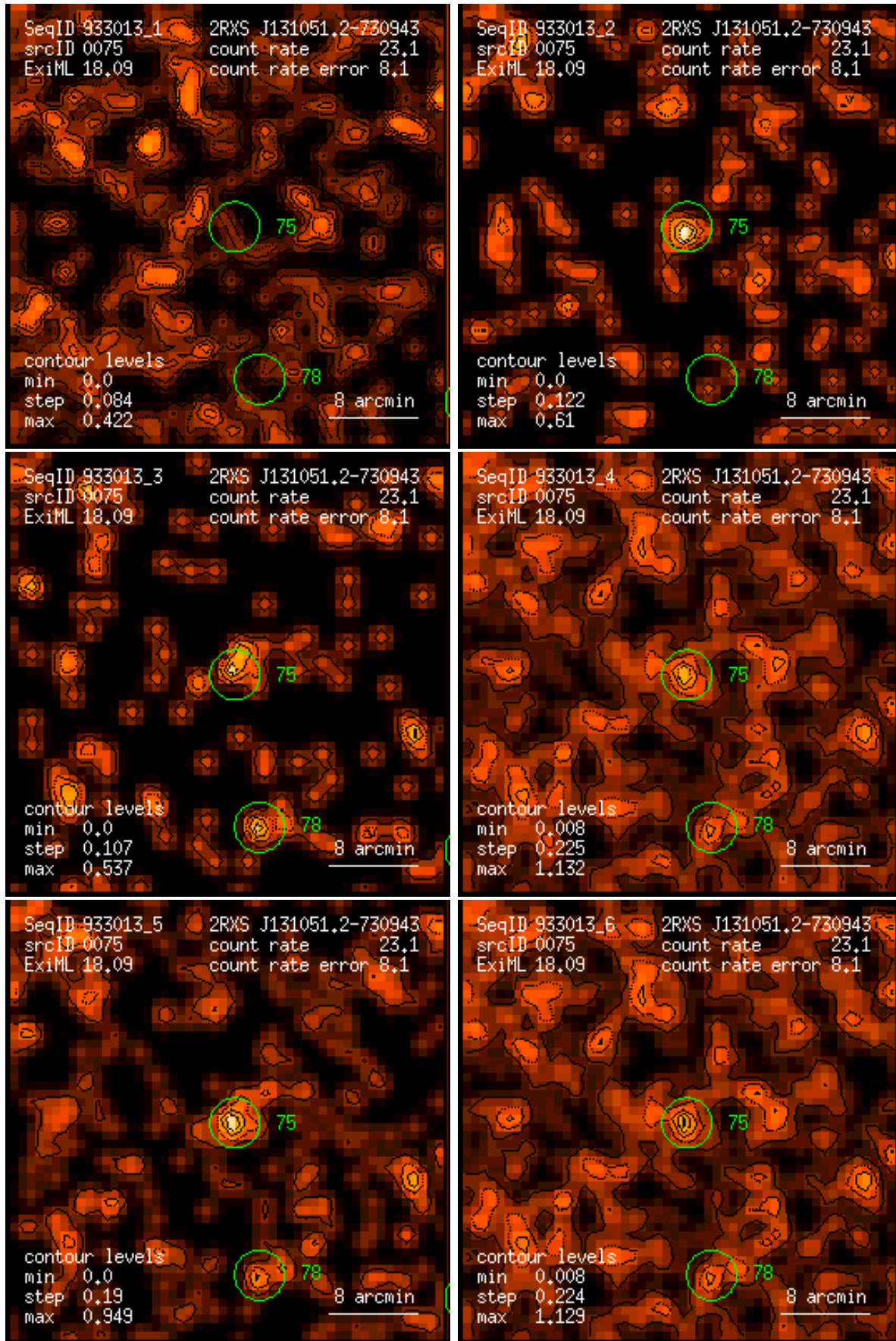
Figure 75: RASS 933013: detection 0075: band rate images, Gaussian filter: (1) PSPC channels 11 – 41, (2) 52 – 90, (3) 91 – 201, (4) 11 – 235, (5) 52 – 201, (6) 11 – 201. Broad band rates in counts/ks. Band rate contour levels in counts/ks/arcmin 2 .
