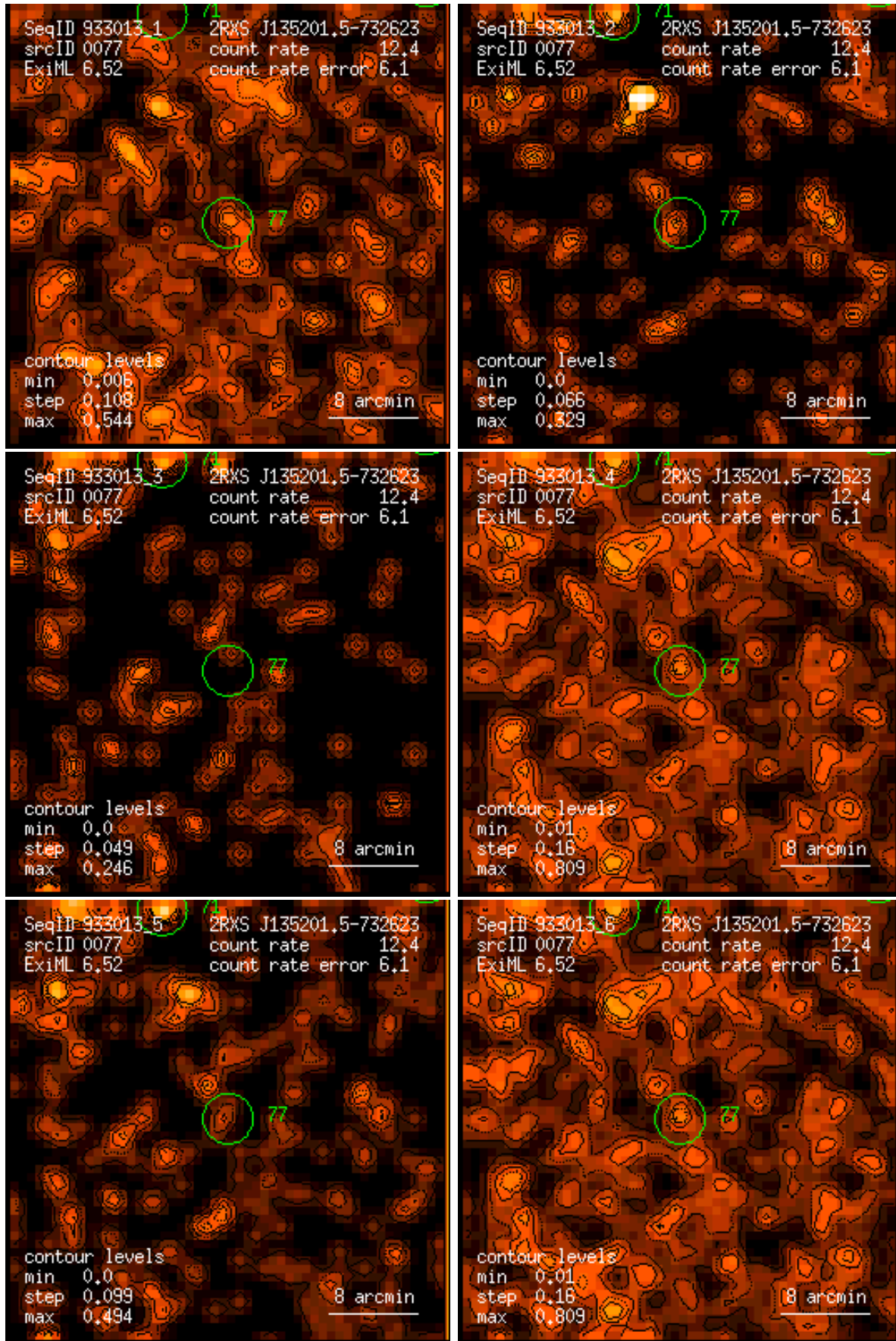
Figure 77: RASS 933013: detection 0077: band rate images, Gaussian filter: (1) PSPC channels 11 – 41, (2) 52 – 90, (3) 91 – 201, (4) 11 – 235, (5) 52 – 201, (6) 11 – 201. Broad band rates in counts/ks. Band rate contour levels in counts/ks/arcmin 2 .
