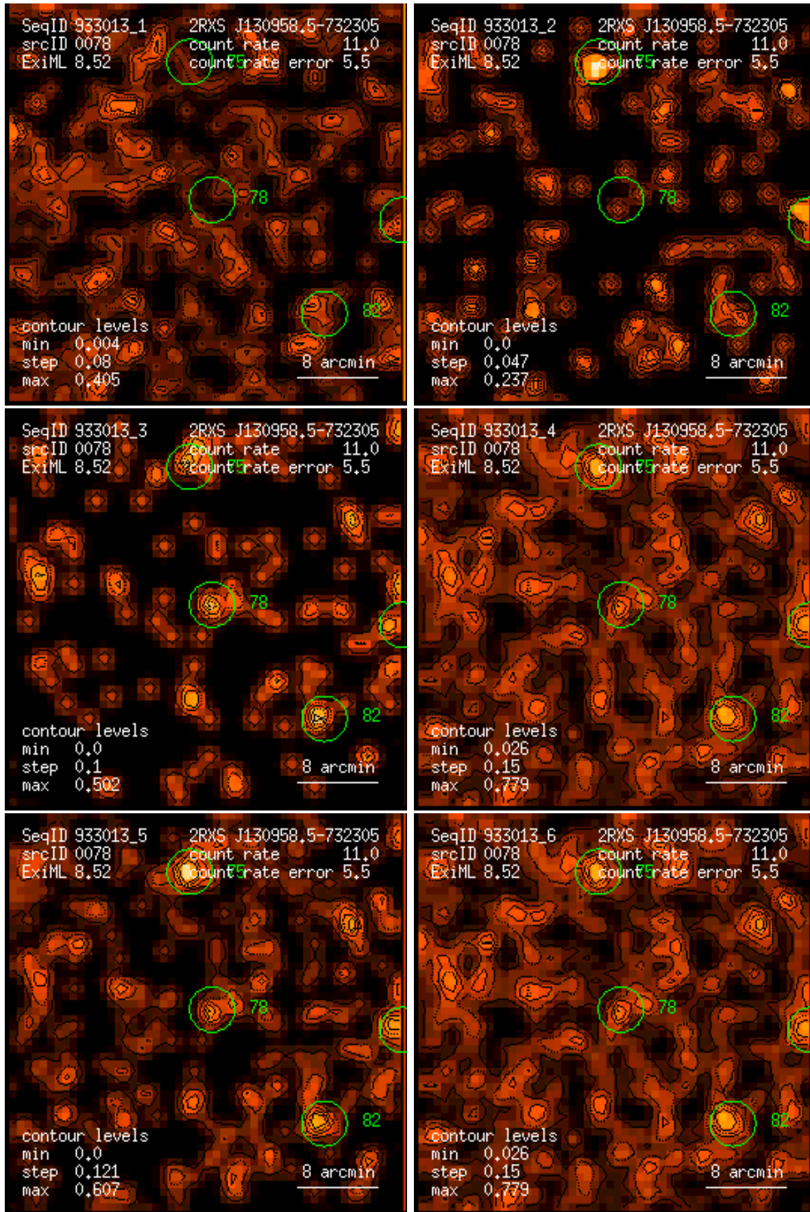
Figure 78: RASS 933013: detection 0078: band rate images, Gaussian filter: (1) PSPC channels 11 – 41, (2) 52 – 90, (3) 91 – 201, (4) 11 – 235, (5) 52 – 201, (6) 11 – 201. Broad band rates in counts/ks. Band rate contour levels in counts/ks/arcmin 2 .
