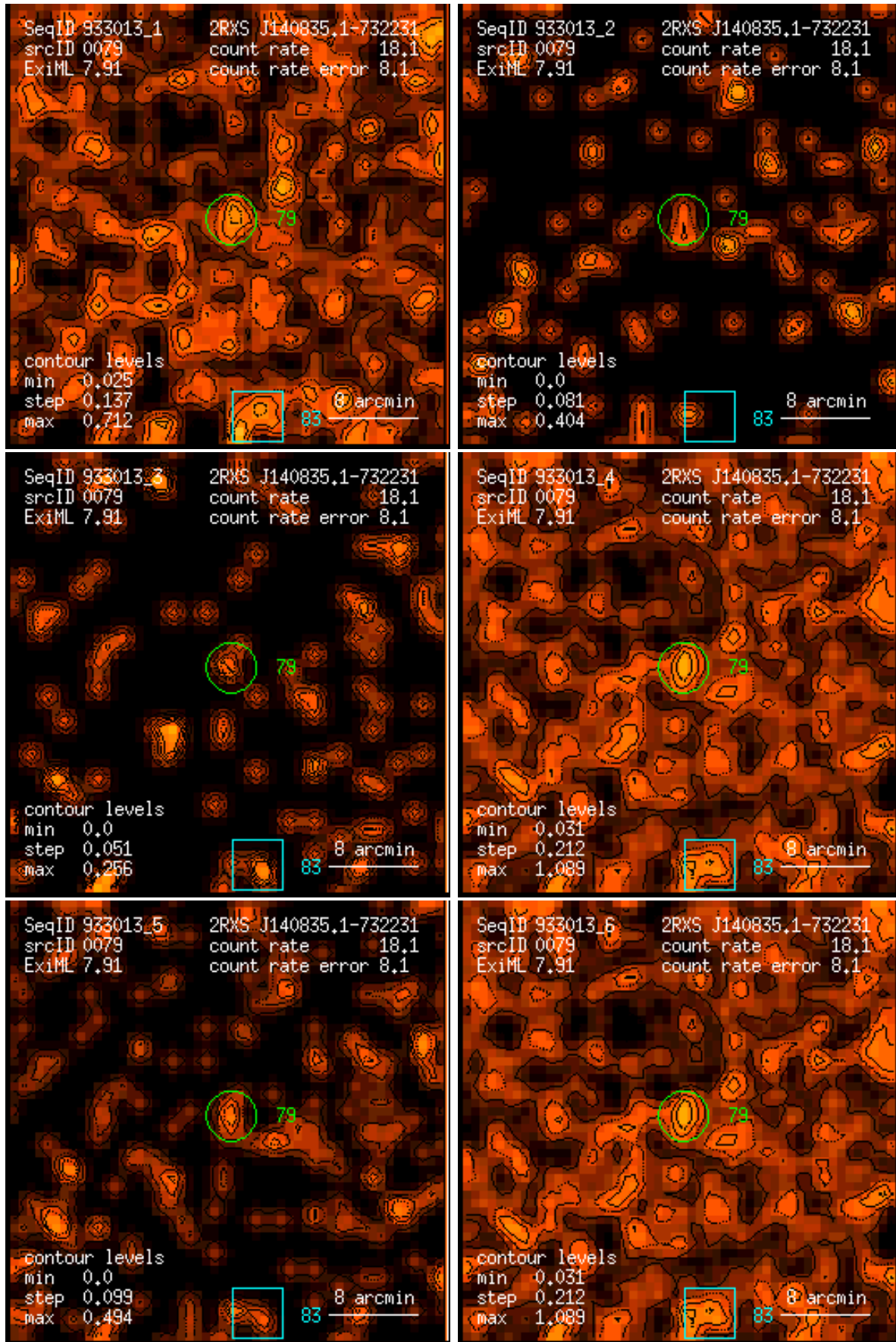
Figure 79: RASS 933013: detection 0079: band rate images, Gaussian filter: (1) PSPC channels 11 – 41, (2) 52 – 90, (3) 91 – 201, (4) 11 – 235, (5) 52 – 201, (6) 11 – 201. Broad band rates in counts/ks. Band rate contour levels in counts/ks/arcmin 2 .
