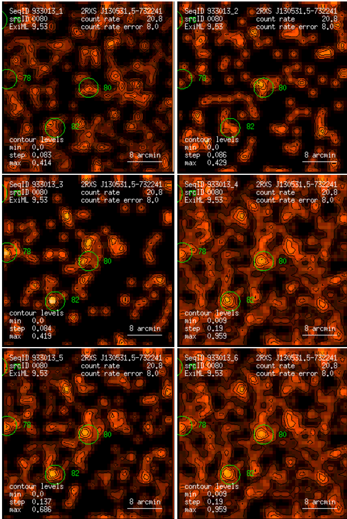
Figure 80: RASS 933013: detection 0080: band rate images, Gaussian filter: (1) PSPC channels 11 – 41, (2) 52 – 90, (3) 91 – 201, (4) 11 – 235, (5) 52 – 201, (6) 11 – 201. Broad band rates in counts/ks. Band rate contour levels in counts/ks/arcmin 2 .
