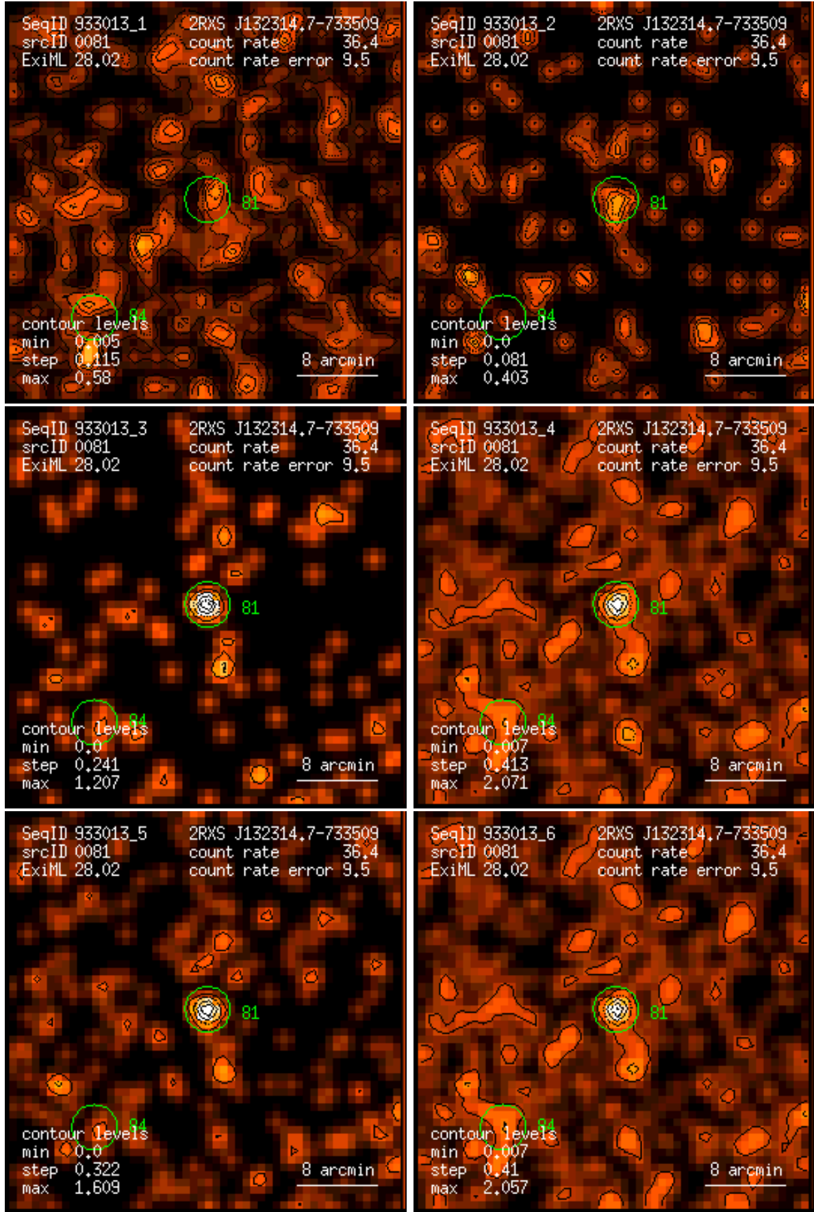
Figure 81: RASS 933013: detection 0081: band rate images, Gaussian filter: (1) PSPC channels 11 – 41, (2) 52 – 90, (3) 91 – 201, (4) 11 – 235, (5) 52 – 201, (6) 11 – 201. Broad band rates in counts/ks. Band rate contour levels in counts/ks/arcmin 2 .
