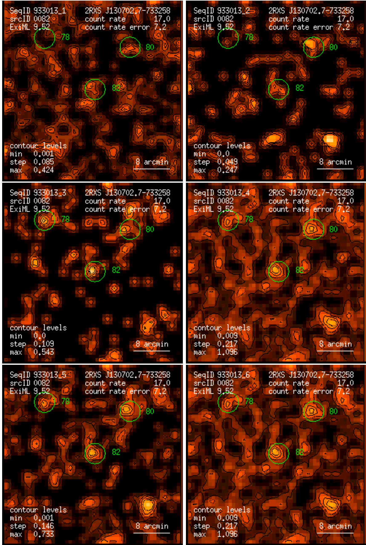
Figure 82: RASS 933013: detection 0082: band rate images, Gaussian filter: (1) PSPC channels 11 – 41, (2) 52 – 90, (3) 91 – 201, (4) 11 – 235, (5) 52 – 201, (6) 11 – 201. Broad band rates in counts/ks. Band rate contour levels in counts/ks/arcmin 2 .
