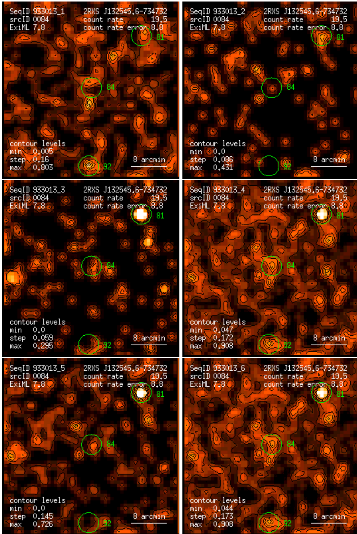
Figure 84: RASS 933013: detection 0084: band rate images, Gaussian filter: (1) PSPC channels 11 – 41, (2) 52 – 90, (3) 91 – 201, (4) 11 – 235, (5) 52 – 201, (6) 11 – 201. Broad band rates in counts/ks. Band rate contour levels in counts/ks/arcmin 2 .
