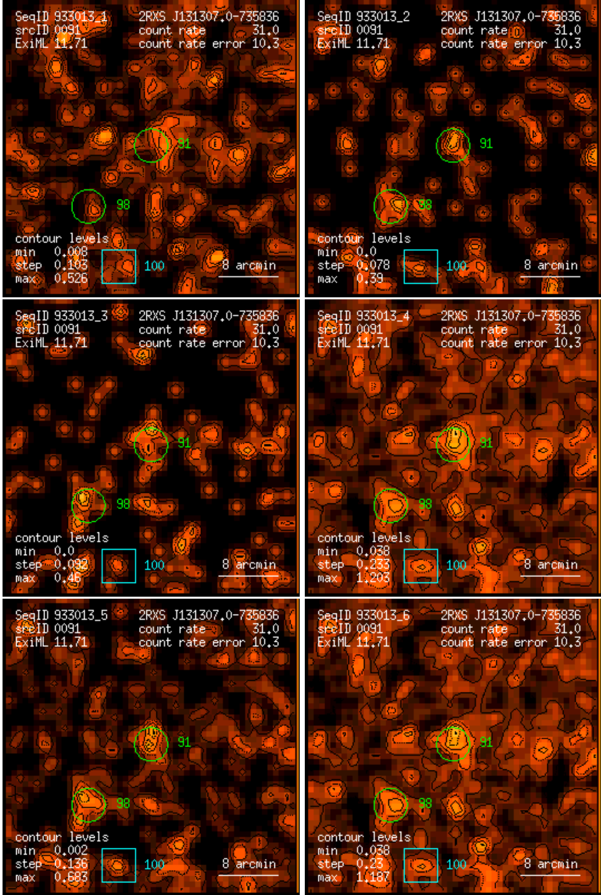
Figure 91: RASS 933013: detection 0091: band rate images, Gaussian filter: (1) PSPC channels 11 – 41, (2) 52 – 90, (3) 91 – 201, (4) 11 – 235, (5) 52 – 201, (6) 11 – 201. Broad band rates in counts/ks. Band rate contour levels in counts/ks/arcmin 2 .
