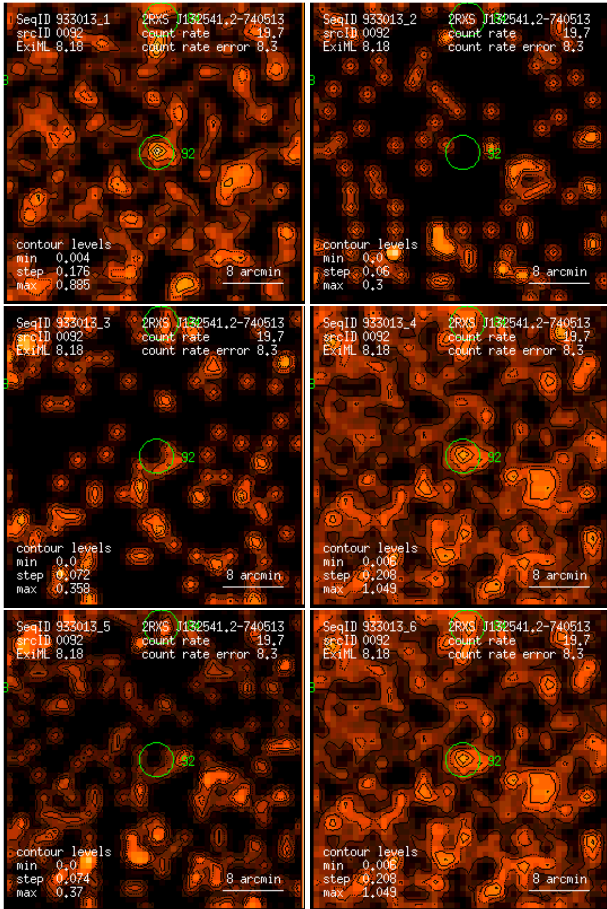
Figure 92: RASS 933013: detection 0092: band rate images, Gaussian filter: (1) PSPC channels 11 – 41, (2) 52 – 90, (3) 91 – 201, (4) 11 – 235, (5) 52 – 201, (6) 11 – 201. Broad band rates in counts/ks. Band rate contour levels in counts/ks/arcmin 2 .
