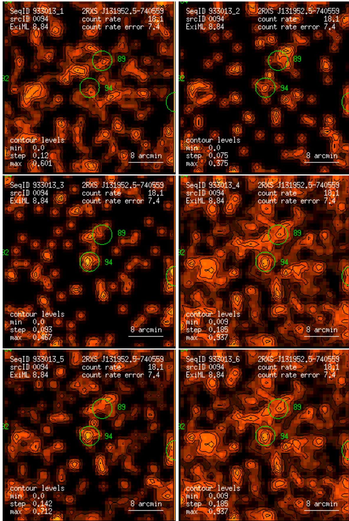
Figure 94: RASS 933013: detection 0094: band rate images, Gaussian filter: (1) PSPC channels 11 – 41, (2) 52 – 90, (3) 91 – 201, (4) 11 – 235, (5) 52 – 201, (6) 11 – 201. Broad band rates in counts/ks. Band rate contour levels in counts/ks/arcmin 2 .
