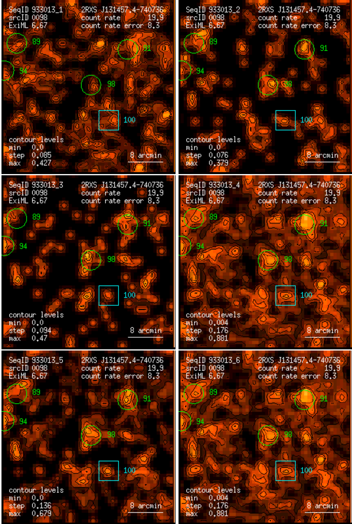
Figure 98: RASS 933013: detection 0098: band rate images, Gaussian filter: (1) PSPC channels 11 – 41, (2) 52 – 90, (3) 91 – 201, (4) 11 – 235, (5) 52 – 201, (6) 11 – 201. Broad band rates in counts/ks. Band rate contour levels in counts/ks/arcmin 2 .
