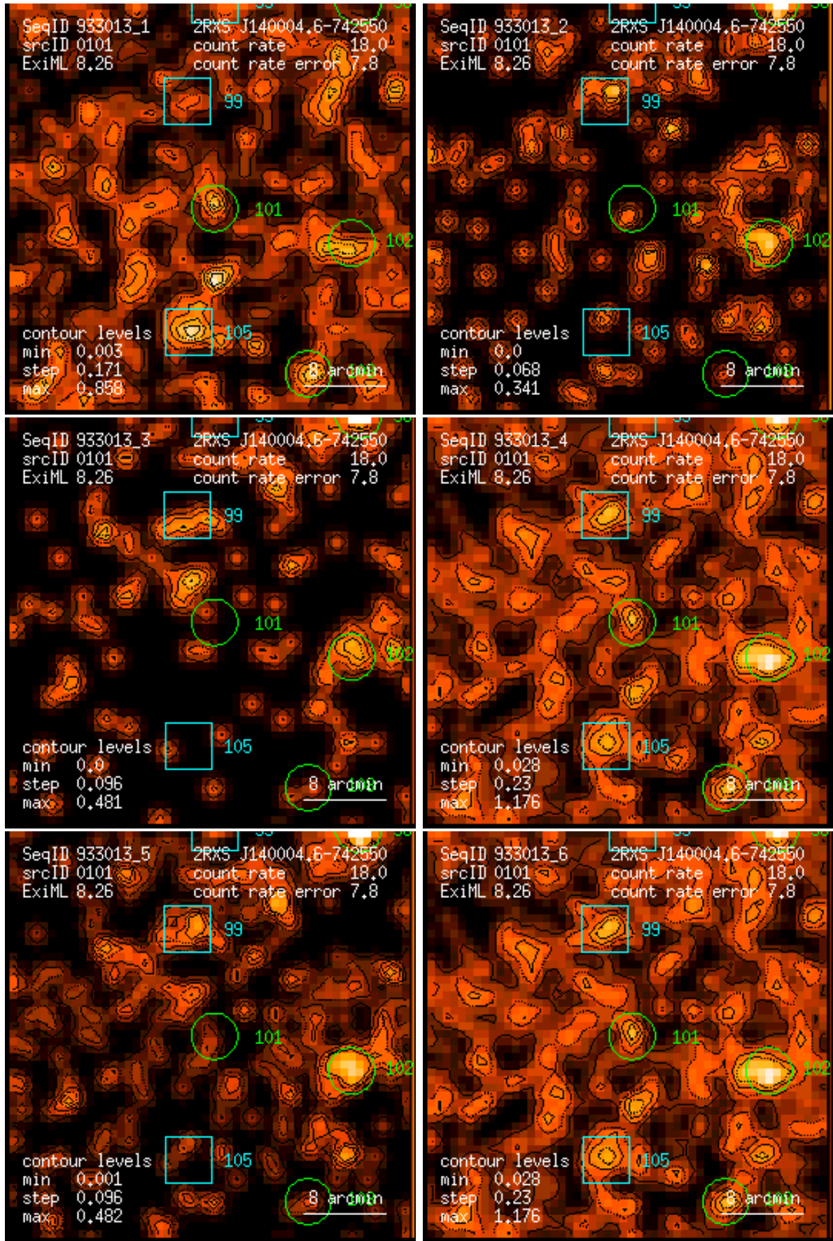
Figure 101: RASS 933013: detection 0101: band rate images, Gaussian filter: (1) PSPC channels 11 – 41, (2) 52 – 90, (3) 91 – 201, (4) 11 – 235, (5) 52 – 201, (6) 11 – 201. Broad band rates in counts/ks. Band rate contour levels in counts/ks/arcmin 2 .
