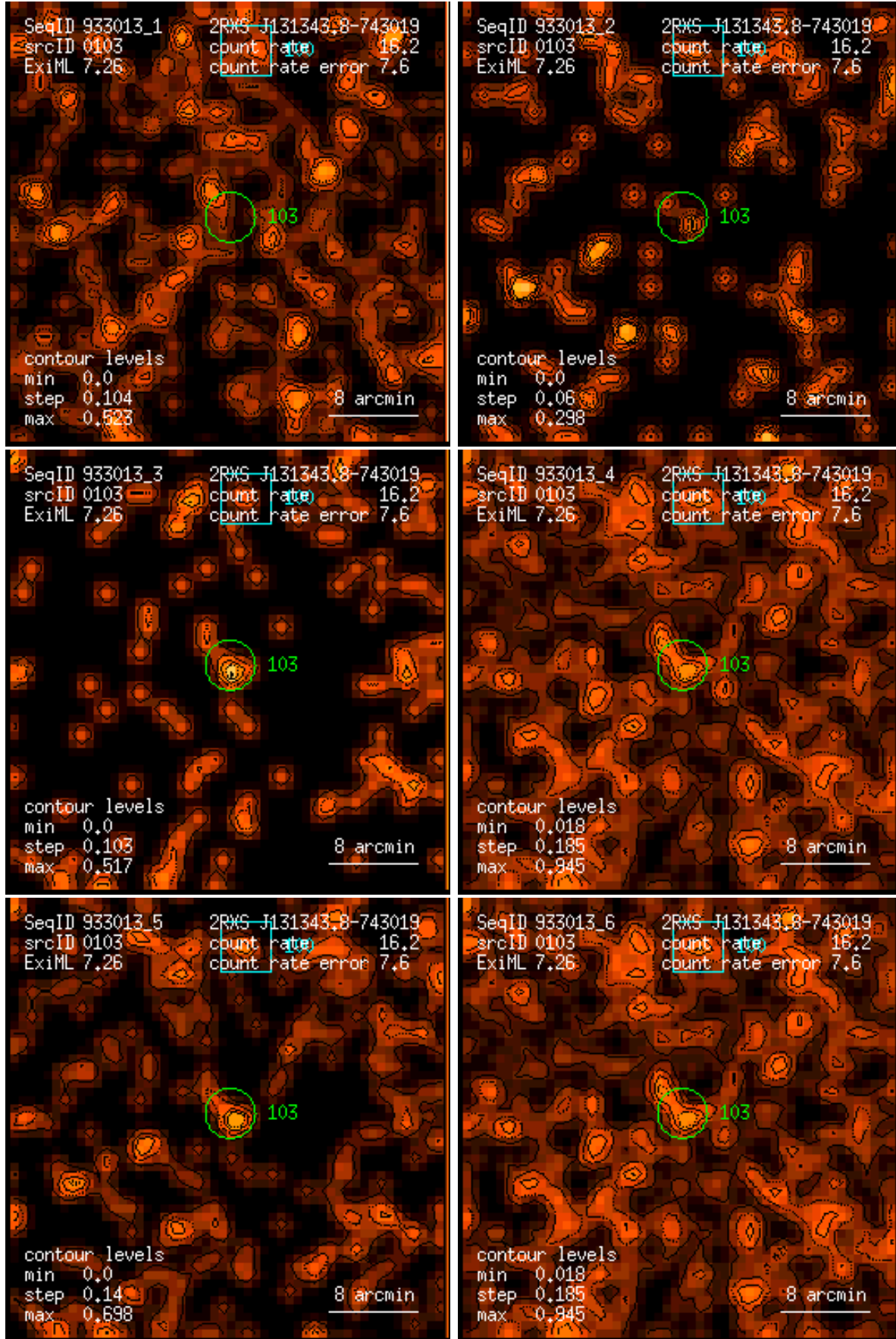
Figure 103: RASS 933013: detection 0103: band rate images, Gaussian filter: (1) PSPC channels 11 – 41, (2) 52 – 90, (3) 91 – 201, (4) 11 – 235, (5) 52 – 201, (6) 11 – 201. Broad band rates in counts/ks. Band rate contour levels in counts/ks/arcmin 2 .
