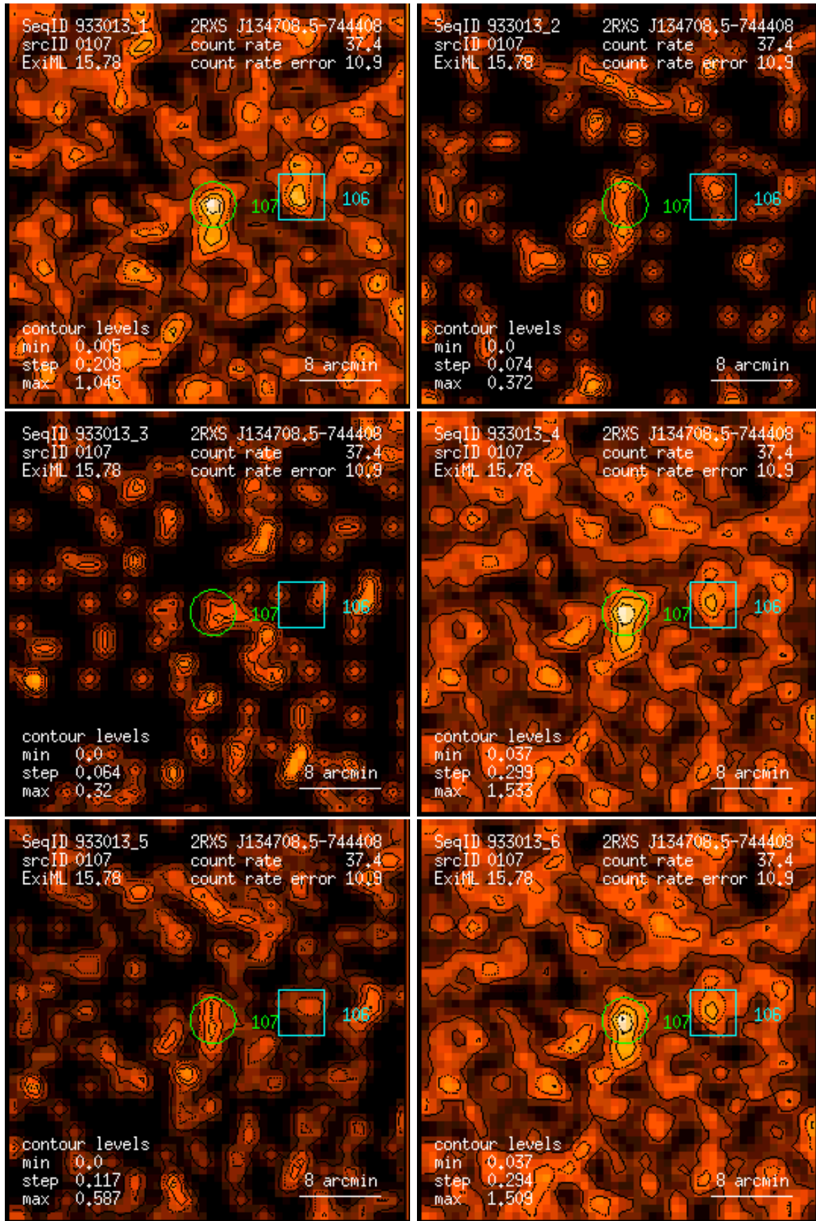
Figure 107: RASS 933013: detection 0107: band rate images, Gaussian filter: (1) PSPC channels 11 – 41, (2) 52 – 90, (3) 91 – 201, (4) 11 – 235, (5) 52 – 201, (6) 11 – 201. Broad band rates in counts/ks. Band rate contour levels in counts/ks/arcmin 2 .
