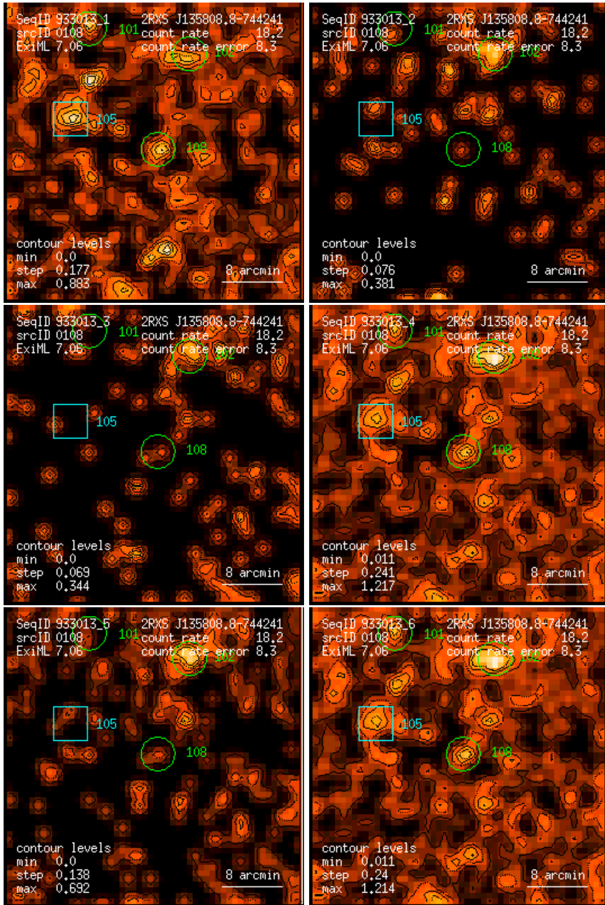
Figure 108: RASS 933013: detection 0108: band rate images, Gaussian filter: (1) PSPC channels 11 – 41, (2) 52 – 90, (3) 91 – 201, (4) 11 – 235, (5) 52 – 201, (6) 11 – 201. Broad band rates in counts/ks. Band rate contour levels in counts/ks/arcmin 2 .
