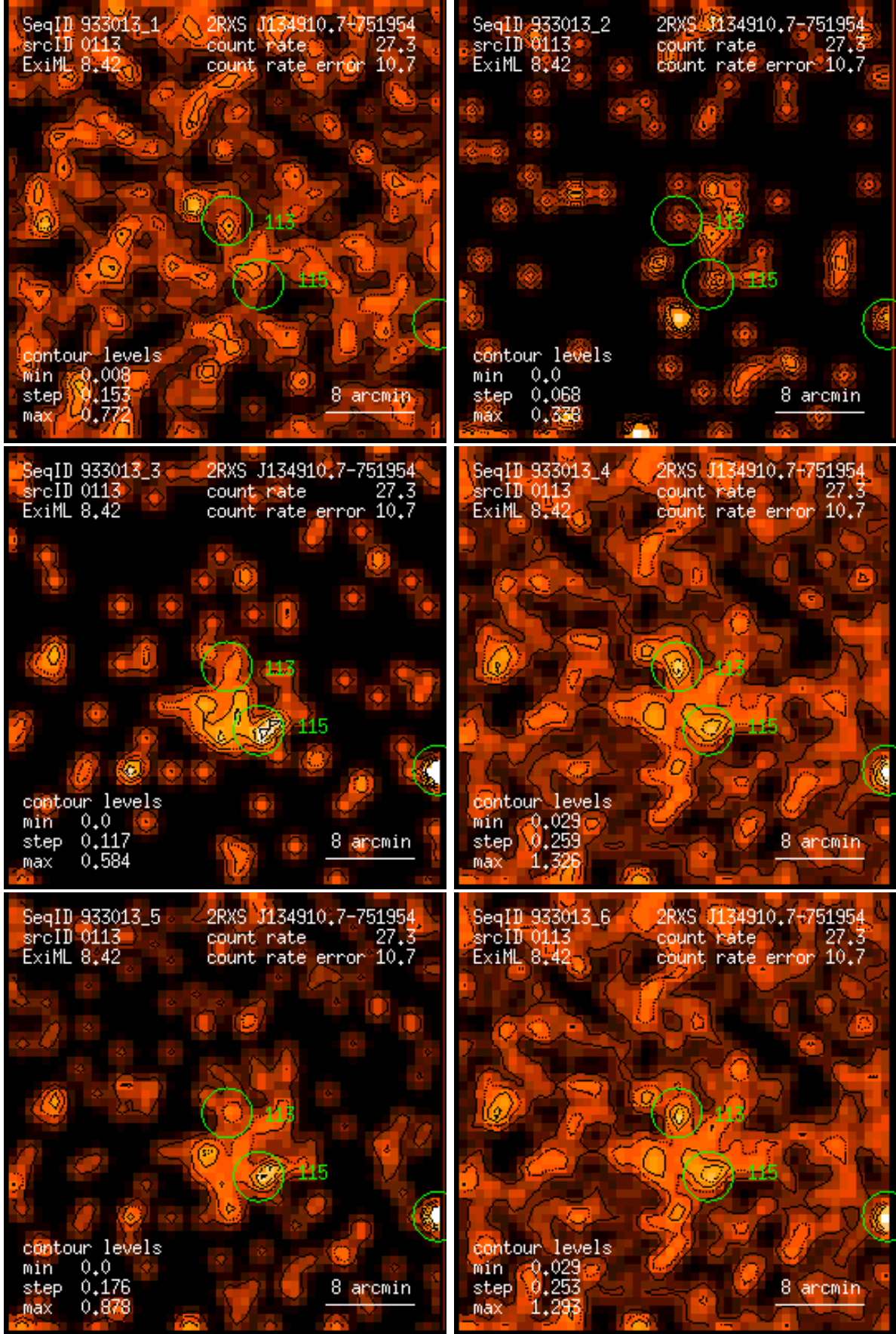
Figure 113: RASS 933013: detection 0113: band rate images, Gaussian filter: (1) PSPC channels 11 – 41, (2) 52 – 90, (3) 91 – 201, (4) 11 – 235, (5) 52 – 201, (6) 11 – 201. Broad band rates in counts/ks. Band rate contour levels in counts/ks/arcmin 2 .
