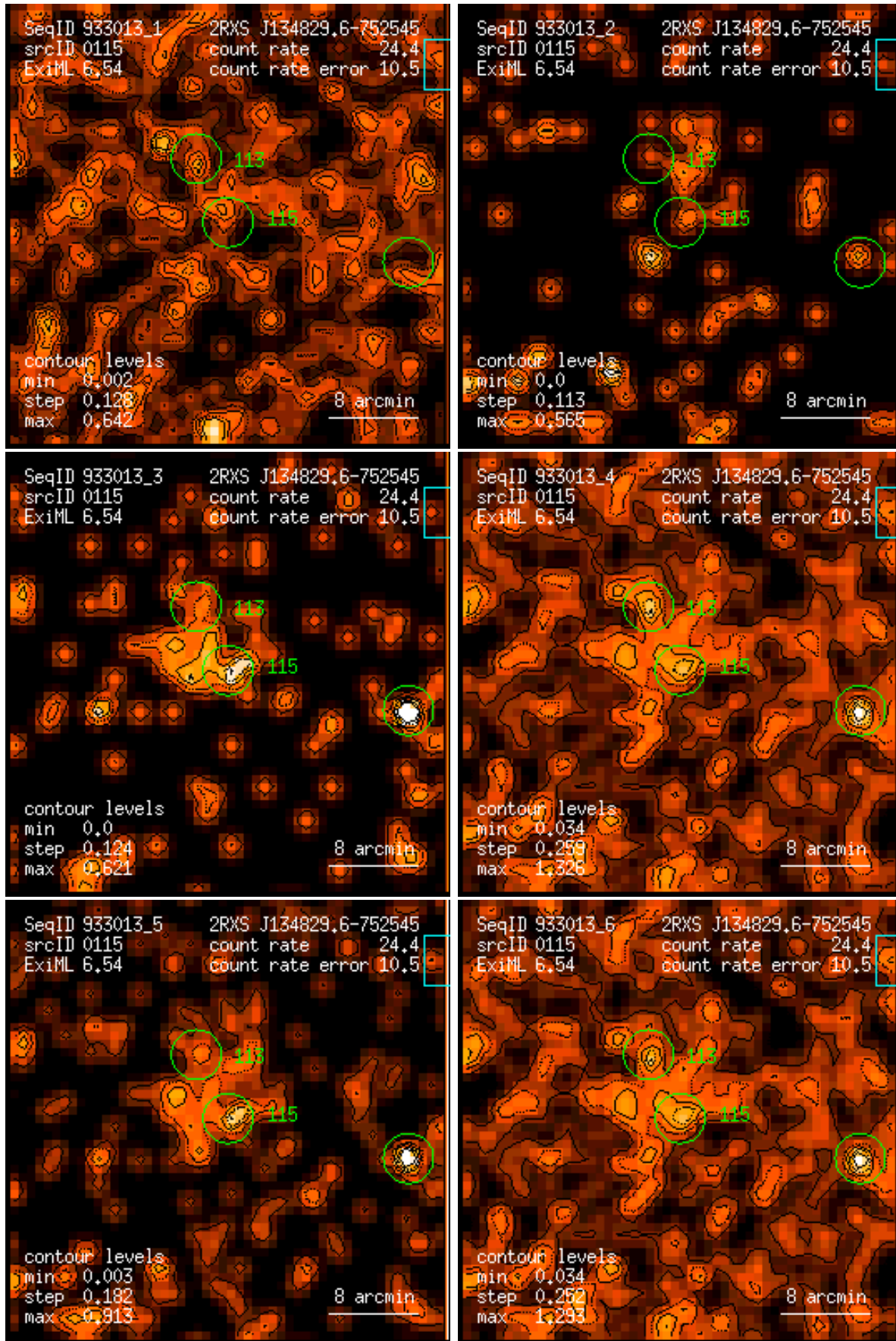
Figure 115: RASS 933013: detection 0115: band rate images, Gaussian filter: (1) PSPC channels 11 – 41, (2) 52 – 90, (3) 91 – 201, (4) 11 – 235, (5) 52 – 201, (6) 11 – 201. Broad band rates in counts/ks. Band rate contour levels in counts/ks/arcmin 2 .
