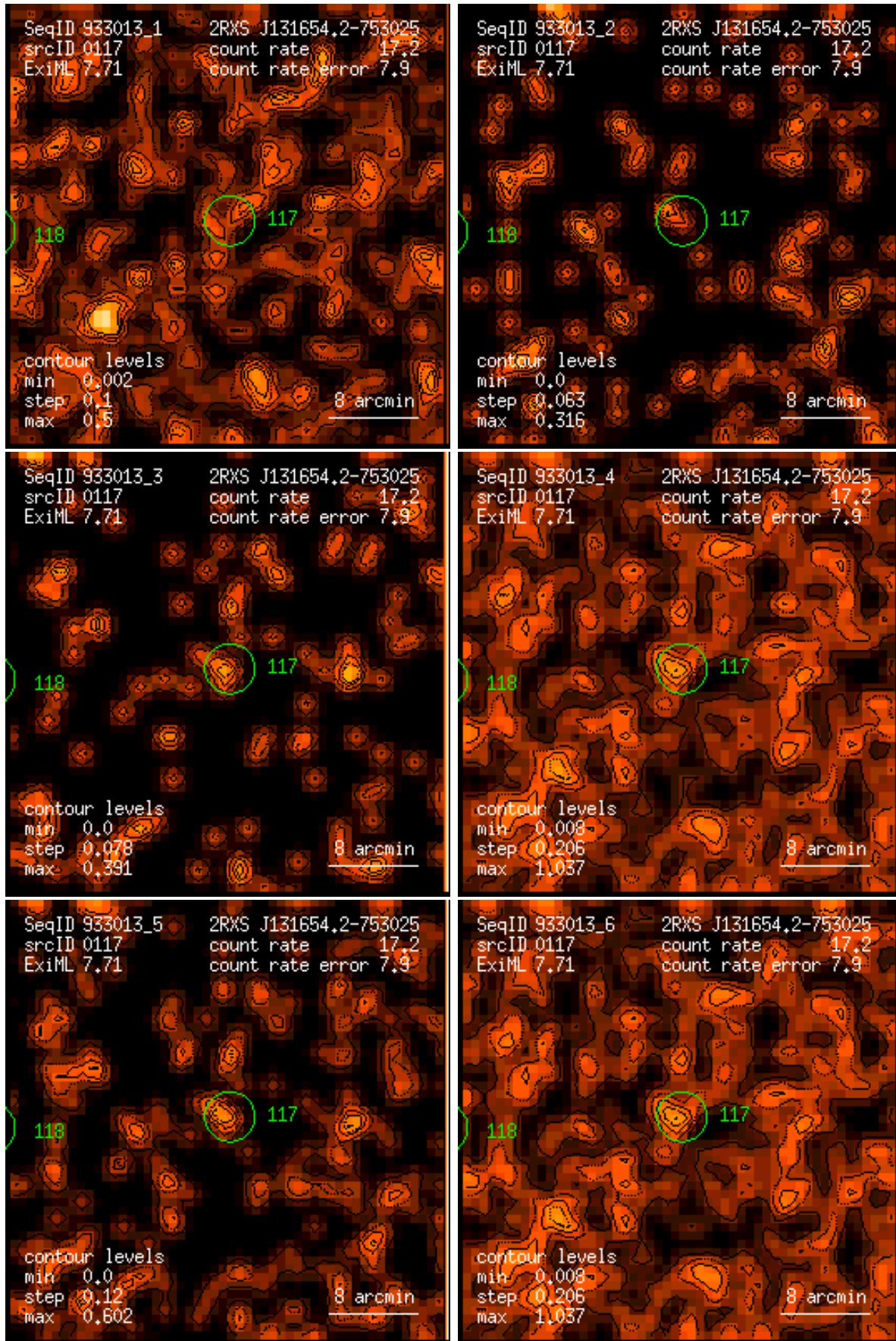
Figure 117: RASS 933013: detection 0117: band rate images, Gaussian filter: (1) PSPC channels 11 – 41, (2) 52 – 90, (3) 91 – 201, (4) 11 – 235, (5) 52 – 201, (6) 11 – 201. Broad band rates in counts/ks. Band rate contour levels in counts/ks/arcmin 2 .
