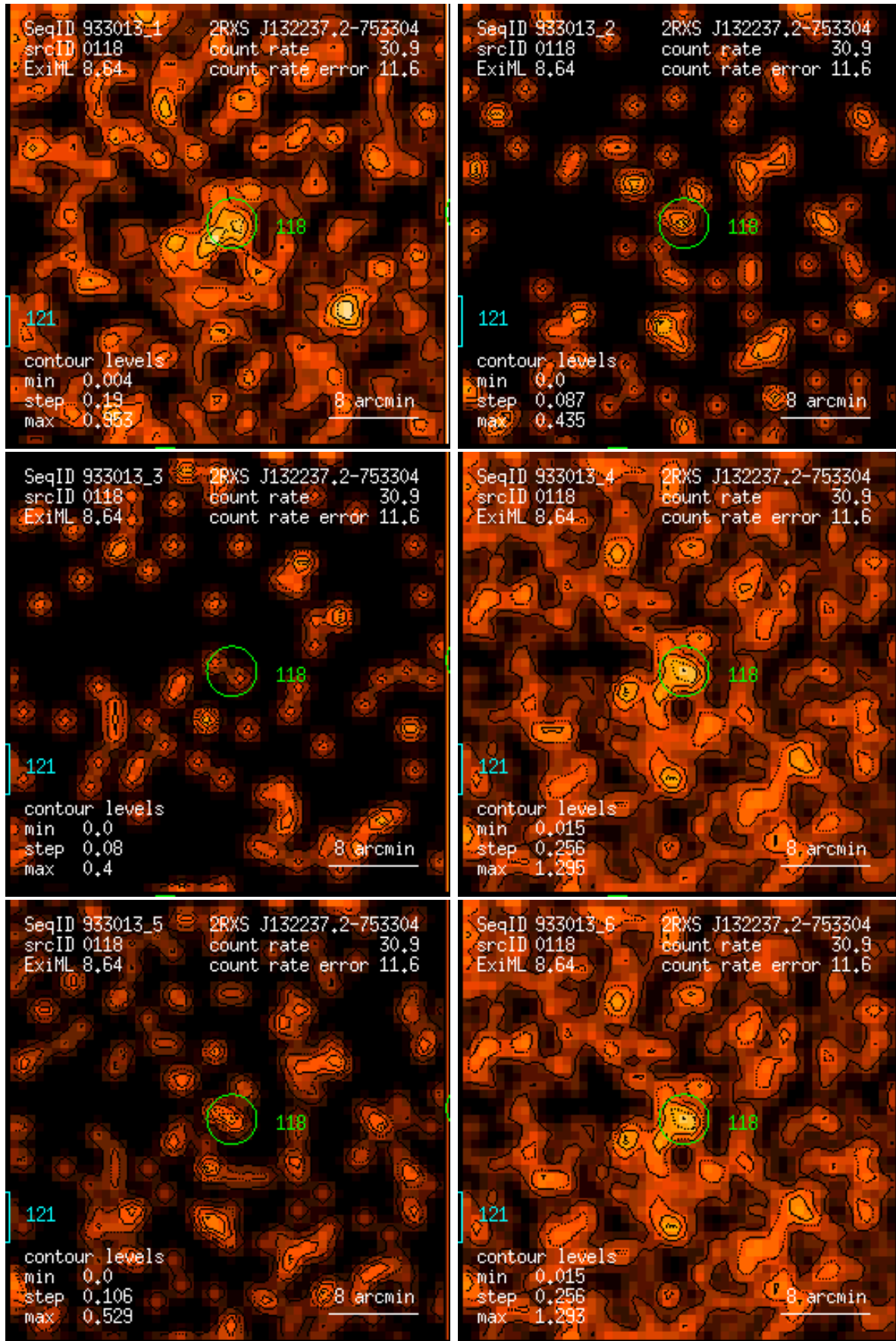
Figure 118: RASS 933013: detection 0118: band rate images, Gaussian filter: (1) PSPC channels 11 – 41, (2) 52 – 90, (3) 91 – 201, (4) 11 – 235, (5) 52 – 201, (6) 11 – 201. Broad band rates in counts/ks. Band rate contour levels in counts/ks/arcmin 2 .
