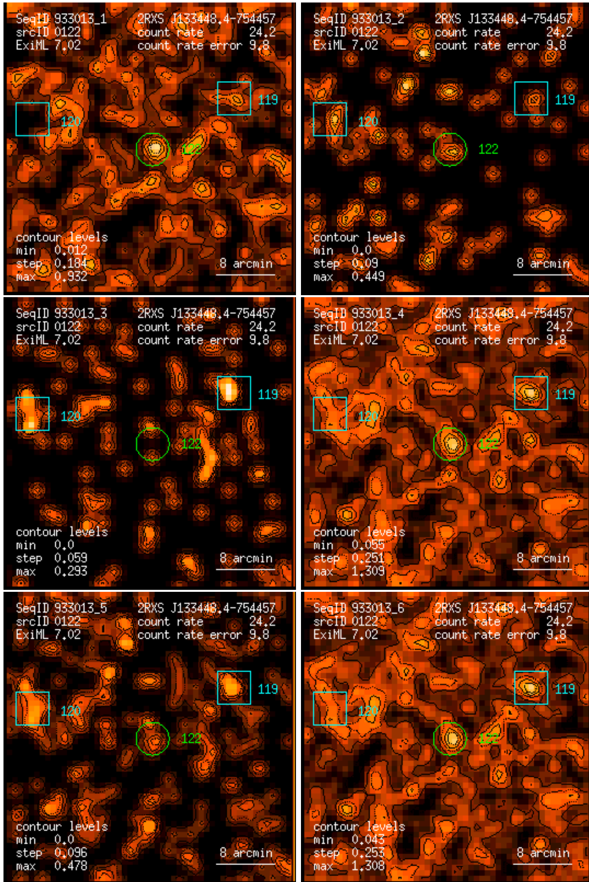
Figure 122: RASS 933013: detection 0122: band rate images, Gaussian filter: (1) PSPC channels 11 – 41, (2) 52 – 90, (3) 91 – 201, (4) 11 – 235, (5) 52 – 201, (6) 11 – 201. Broad band rates in counts/ks. Band rate contour levels in counts/ks/arcmin 2 .
