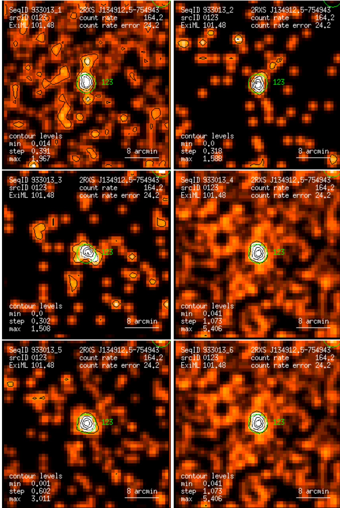
Figure 123: RASS 933013: detection 0123: band rate images, Gaussian filter: (1) PSPC channels 11 – 41, (2) 52 – 90, (3) 91 – 201, (4) 11 – 235, (5) 52 – 201, (6) 11 – 201. Broad band rates in counts/ks. Band rate contour levels in counts/ks/arcmin 2 .
