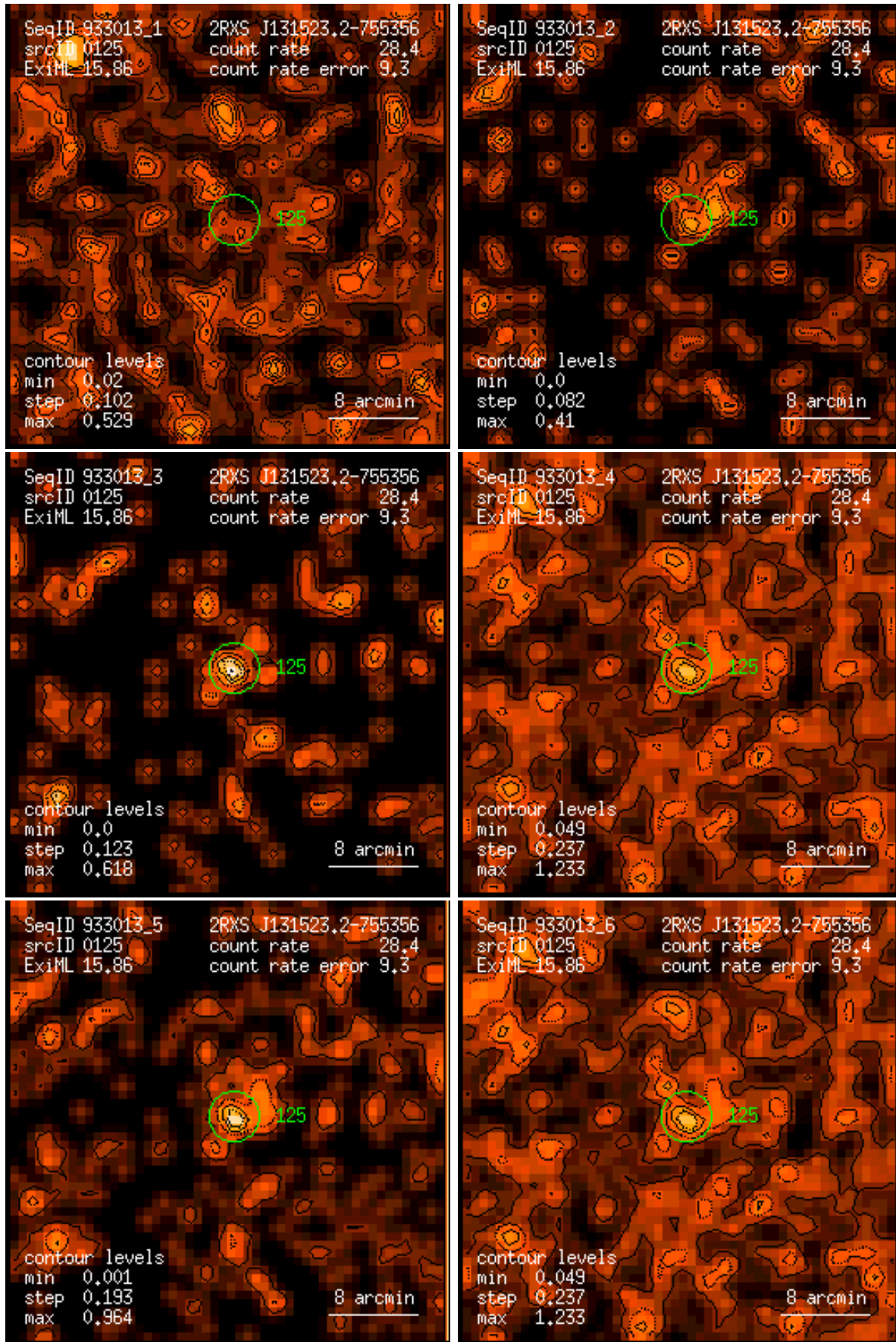
Figure 125: RASS 933013: detection 0125: band rate images, Gaussian filter: (1) PSPC channels 11 – 41, (2) 52 – 90, (3) 91 – 201, (4) 11 – 235, (5) 52 – 201, (6) 11 – 201. Broad band rates in counts/ks. Band rate contour levels in counts/ks/arcmin 2 .
