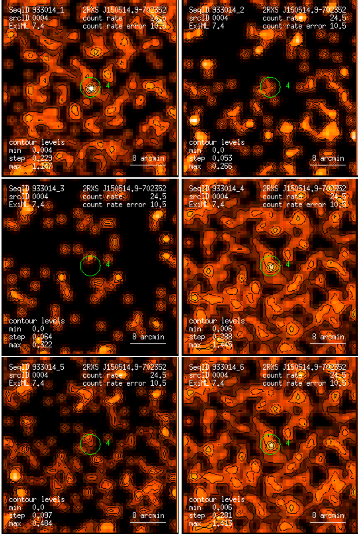
Figure 4: RASS 933014: detection 0004: band rate images, Gaussian filter: (1) PSPC channels 11 – 41, (2) 52 – 90, (3) 91 – 201, (4) 11 – 235, (5) 52 – 201, (6) 11 – 201. Broad band rates in counts/ks. Band rate contour levels in counts/ks/arcmin 2 .
