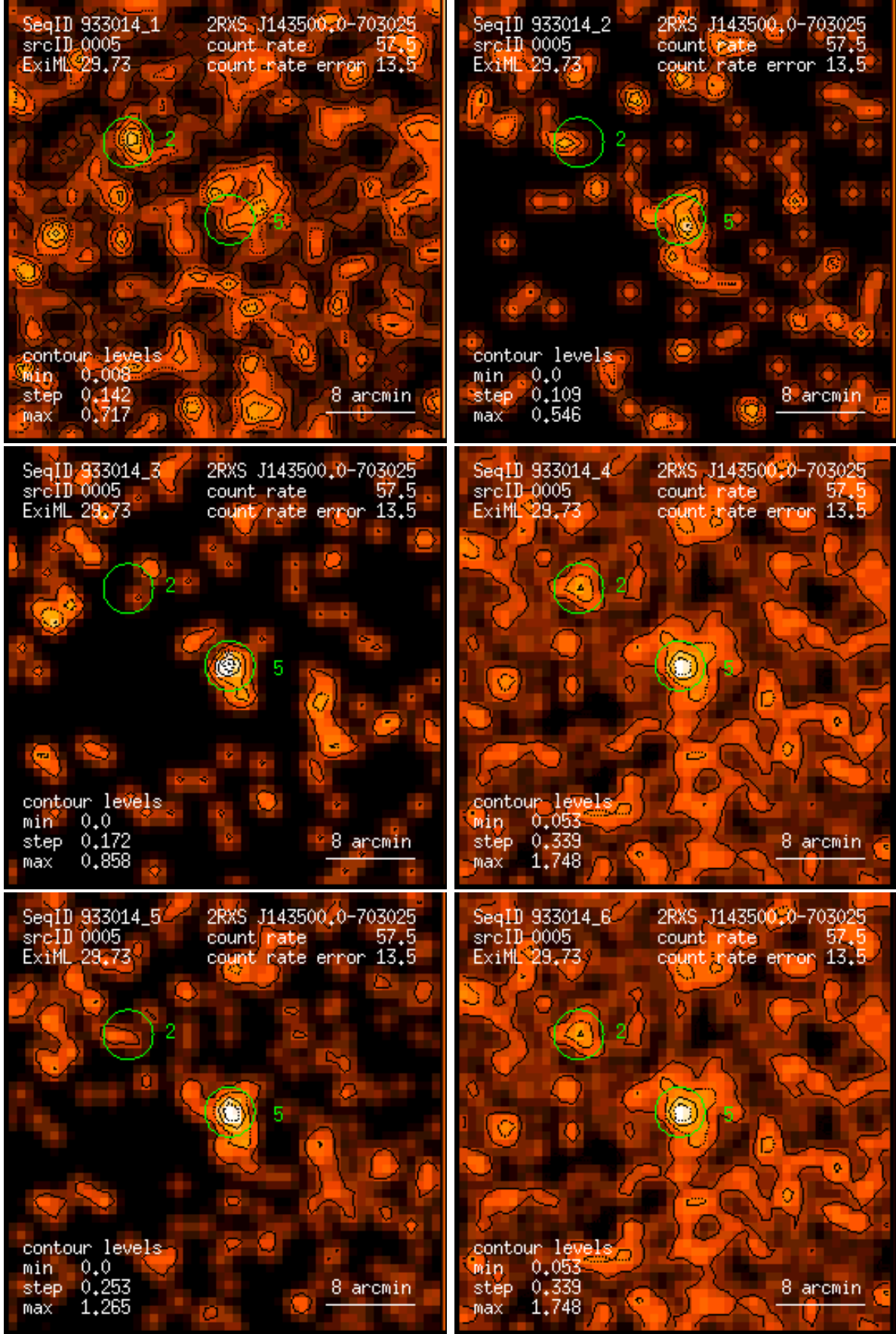
Figure 5: RASS 933014: detection 0005: band rate images, Gaussian filter: (1) PSPC channels 11 – 41, (2) 52 – 90, (3) 91 – 201, (4) 11 – 235, (5) 52 – 201, (6) 11 – 201. Broad band rates in counts/ks. Band rate contour levels in counts/ks/arcmin 2 .
