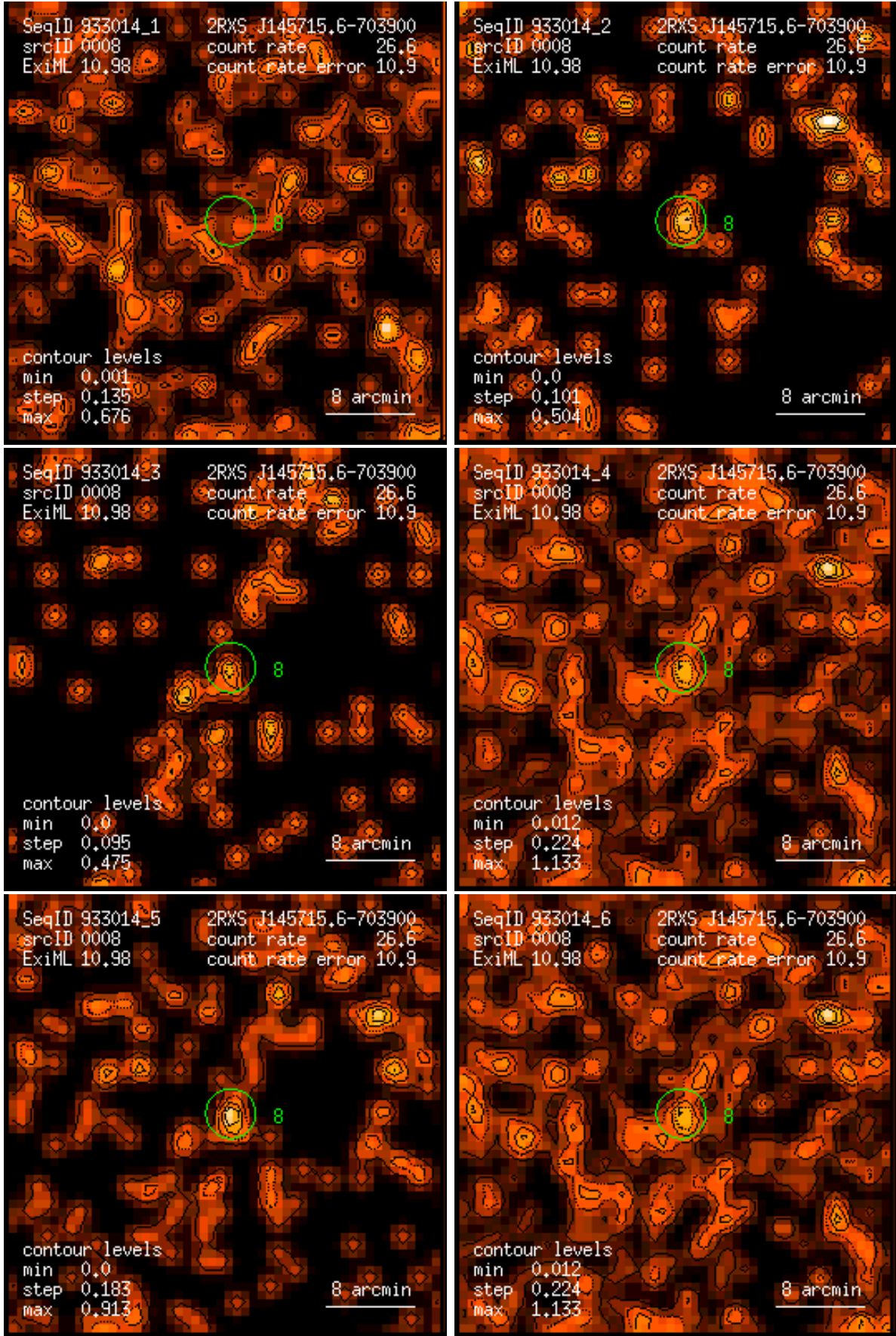
Figure 8: RASS 933014: detection 0008: band rate images, Gaussian filter: (1) PSPC channels 11 – 41, (2) 52 – 90, (3) 91 – 201, (4) 11 – 235, (5) 52 – 201, (6) 11 – 201. Broad band rates in counts/ks. Band rate contour levels in counts/ks/arcmin 2 .
