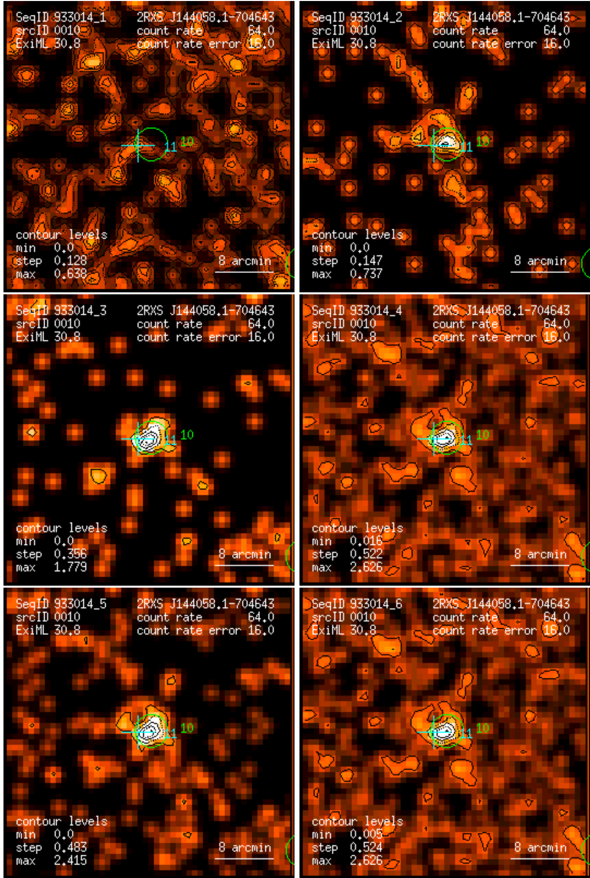
Figure 10: RASS 933014: detection 0010: band rate images, Gaussian filter: (1) PSPC channels 11 – 41, (2) 52 – 90, (3) 91 – 201, (4) 11 – 235, (5) 52 – 201, (6) 11 – 201. Broad band rates in counts/ks. Band rate contour levels in counts/ks/arcmin 2 .
