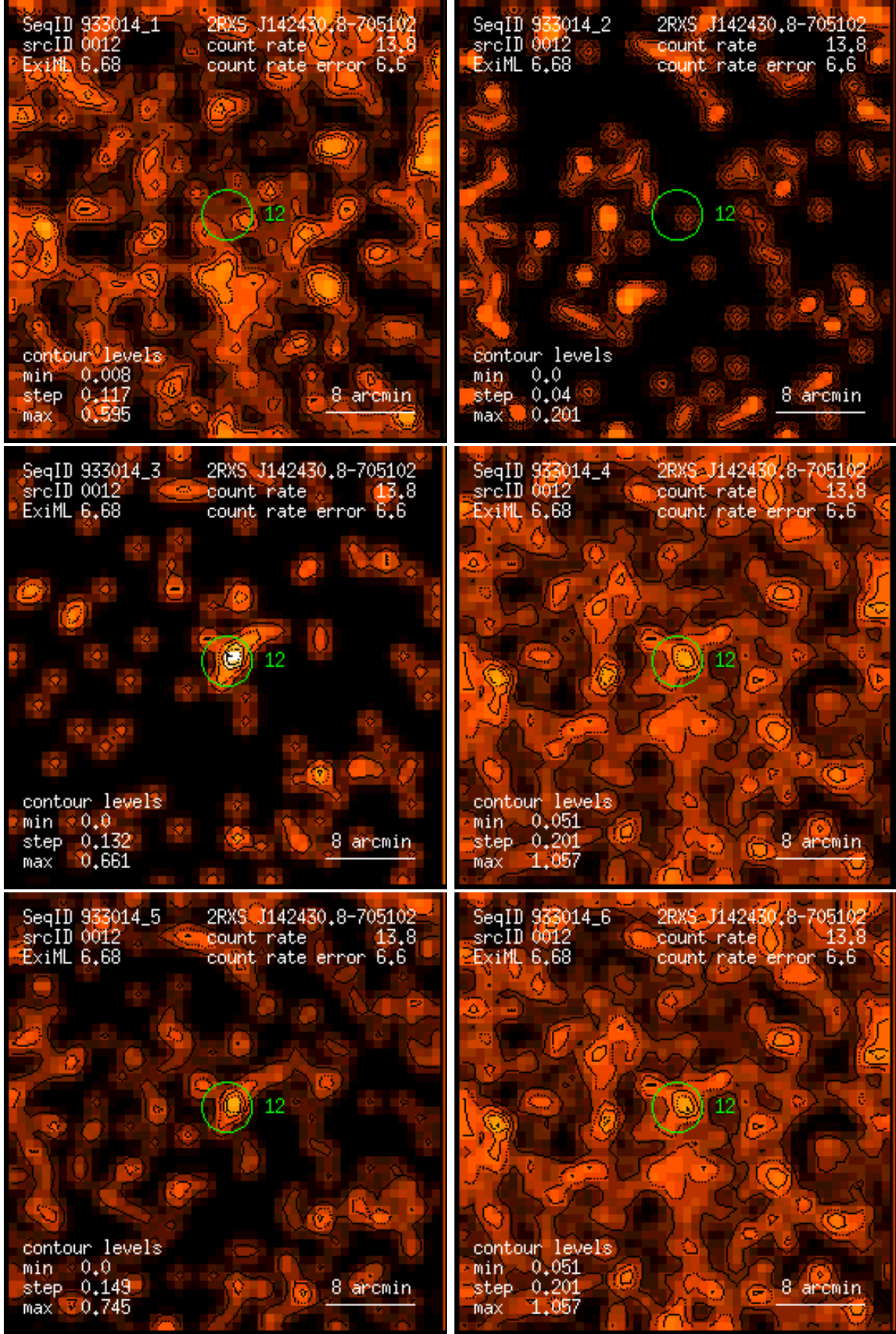
Figure 12: RASS 933014: detection 0012: band rate images, Gaussian filter: (1) PSPC channels 11 – 41, (2) 52 – 90, (3) 91 – 201, (4) 11 – 235, (5) 52 – 201, (6) 11 – 201. Broad band rates in counts/ks. Band rate contour levels in counts/ks/arcmin 2 .
