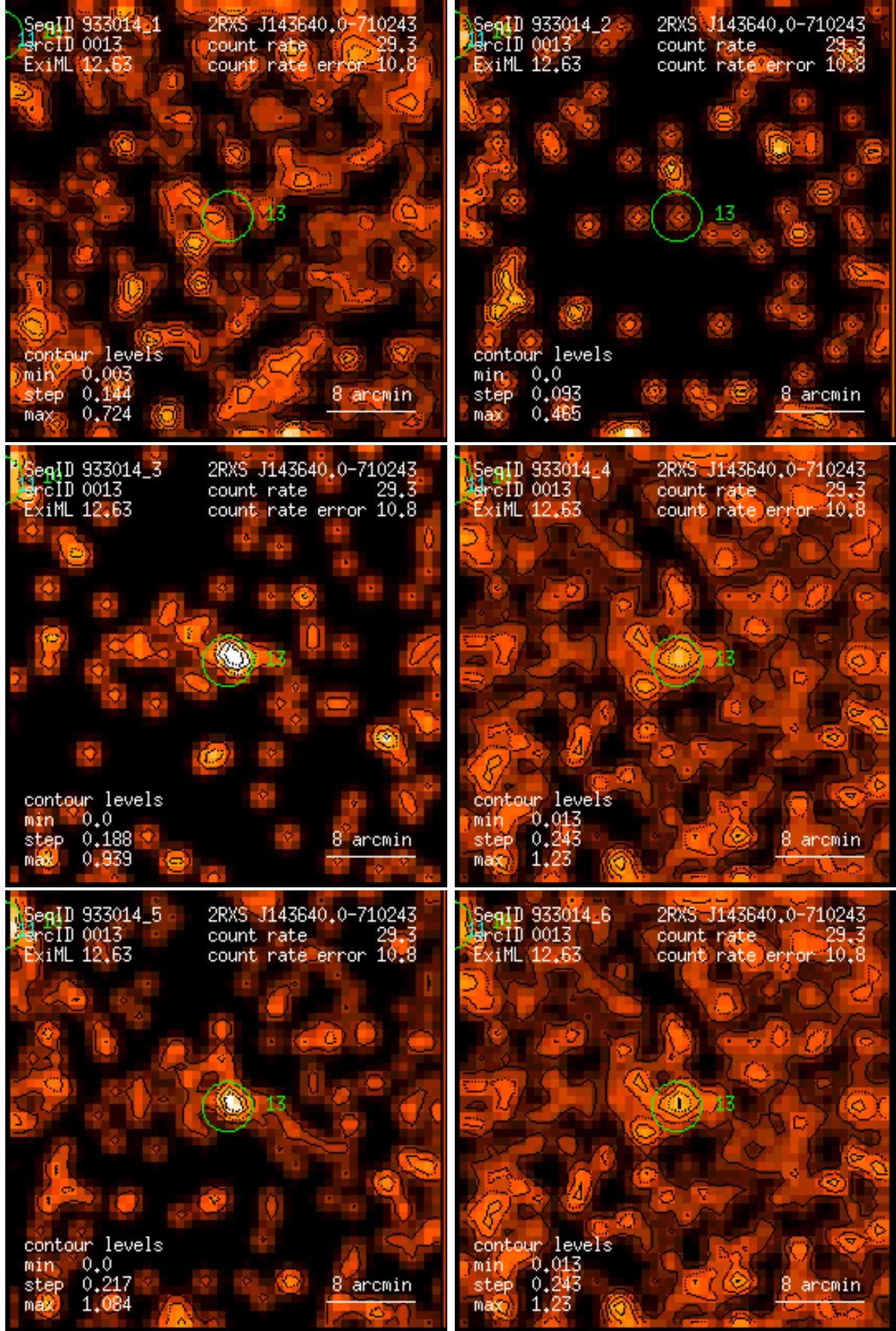
Figure 13: RASS 933014: detection 0013: band rate images, Gaussian filter: (1) PSPC channels 11 – 41, (2) 52 – 90, (3) 91 – 201, (4) 11 – 235, (5) 52 – 201, (6) 11 – 201. Broad band rates in counts/ks. Band rate contour levels in counts/ks/arcmin 2 .
