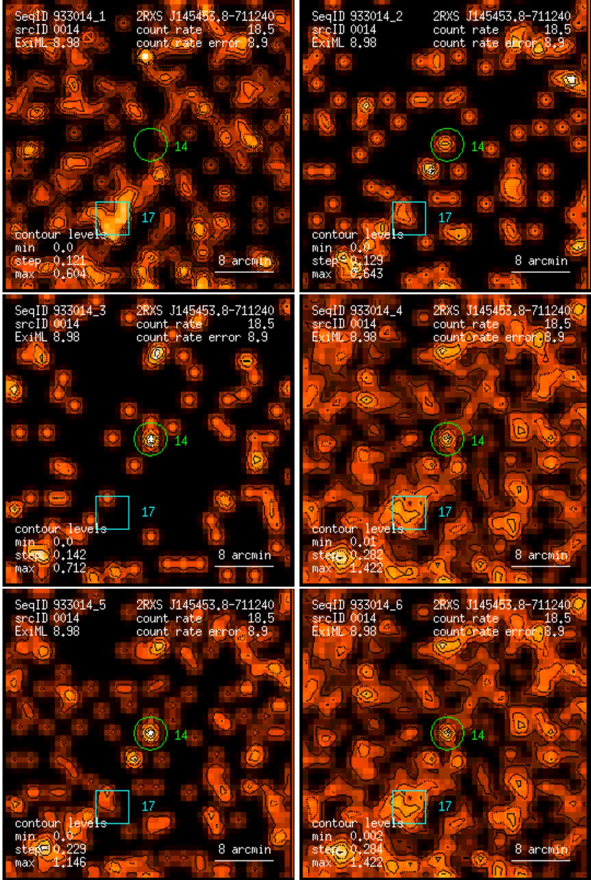
Figure 14: RASS 933014: detection 0014: band rate images, Gaussian filter: (1) PSPC channels 11 – 41, (2) 52 – 90, (3) 91 – 201, (4) 11 – 235, (5) 52 – 201, (6) 11 – 201. Broad band rates in counts/ks. Band rate contour levels in counts/ks/arcmin 2 .
