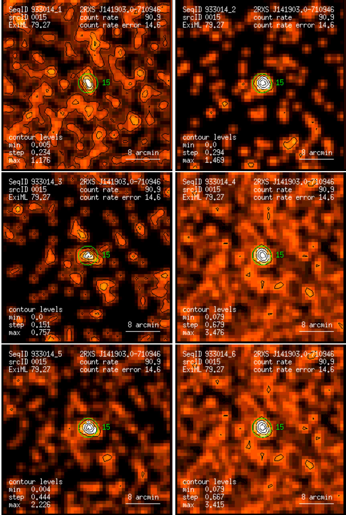
Figure 15: RASS 933014: detection 0015: band rate images, Gaussian filter: (1) PSPC channels 11 – 41, (2) 52 – 90, (3) 91 – 201, (4) 11 – 235, (5) 52 – 201, (6) 11 – 201. Broad band rates in counts/ks. Band rate contour levels in counts/ks/arcmin 2 .
