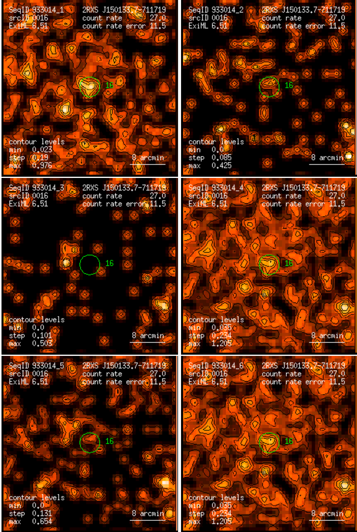
Figure 16: RASS 933014: detection 0016: band rate images, Gaussian filter: (1) PSPC channels 11 – 41, (2) 52 – 90, (3) 91 – 201, (4) 11 – 235, (5) 52 – 201, (6) 11 – 201. Broad band rates in counts/ks. Band rate contour levels in counts/ks/arcmin 2 .
