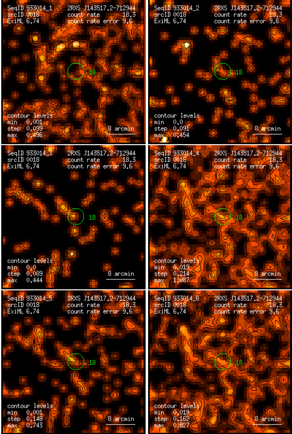
Figure 18: RASS 933014: detection 0018: band rate images, Gaussian filter: (1) PSPC channels 11 – 41, (2) 52 – 90, (3) 91 – 201, (4) 11 – 235, (5) 52 – 201, (6) 11 – 201. Broad band rates in counts/ks. Band rate contour levels in counts/ks/arcmin 2 .
