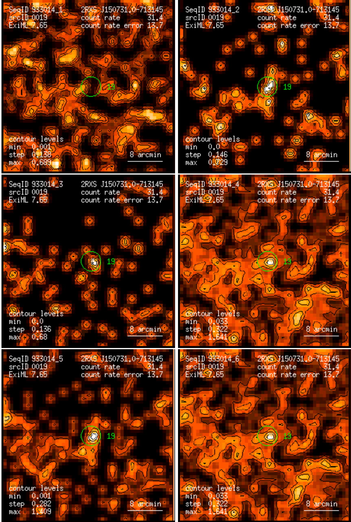
Figure 19: RASS 933014: detection 0019: band rate images, Gaussian filter: (1) PSPC channels 11 – 41, (2) 52 – 90, (3) 91 – 201, (4) 11 – 235, (5) 52 – 201, (6) 11 – 201. Broad band rates in counts/ks. Band rate contour levels in counts/ks/arcmin 2 .
