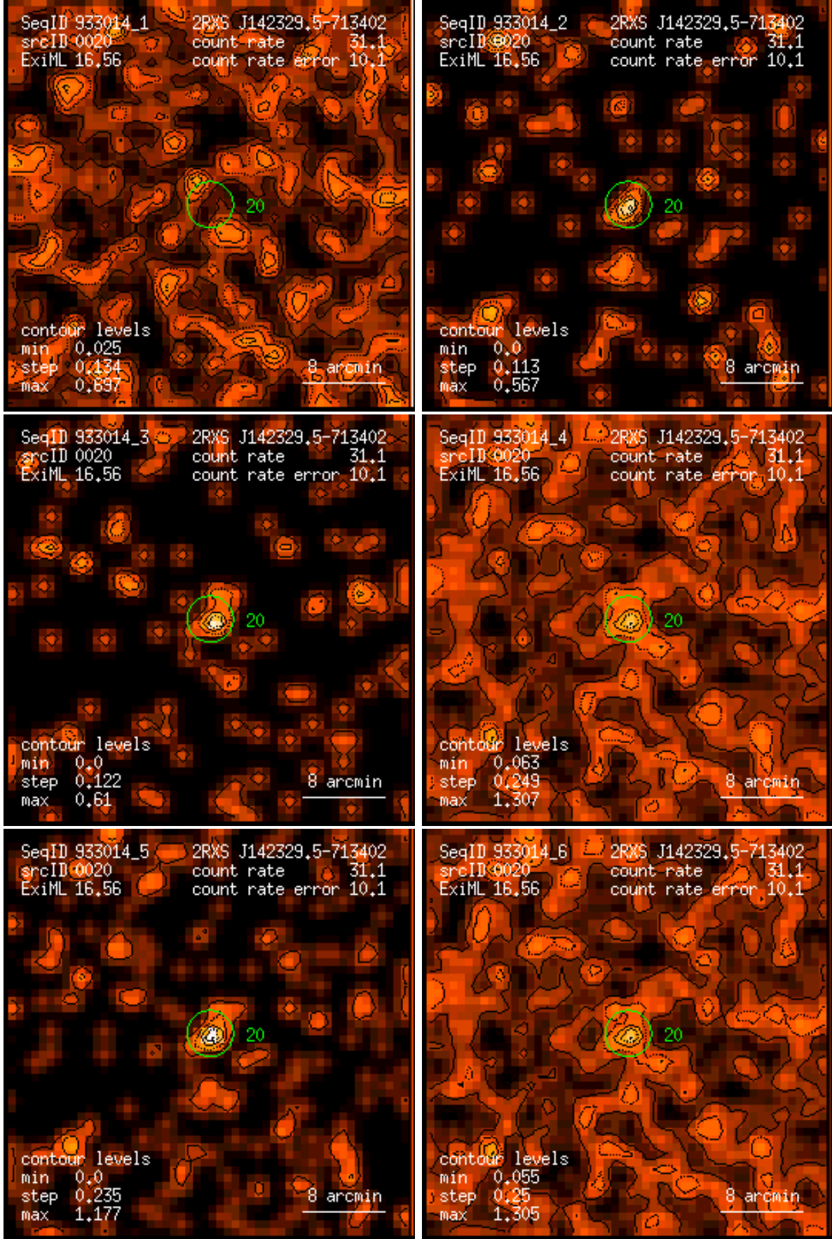
Figure 20: RASS 933014: detection 0020: band rate images, Gaussian filter: (1) PSPC channels 11 – 41, (2) 52 – 90, (3) 91 – 201, (4) 11 – 235, (5) 52 – 201, (6) 11 – 201. Broad band rates in counts/ks. Band rate contour levels in counts/ks/arcmin 2 .
