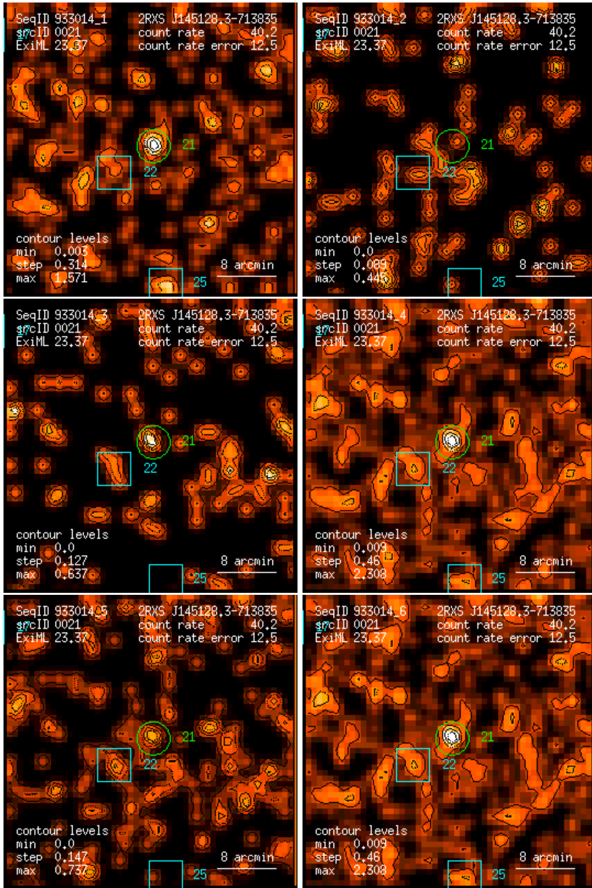
Figure 21: RASS 933014: detection 0021: band rate images, Gaussian filter: (1) PSPC channels 11 – 41, (2) 52 – 90, (3) 91 – 201, (4) 11 – 235, (5) 52 – 201, (6) 11 – 201. Broad band rates in counts/ks. Band rate contour levels in counts/ks/arcmin 2 .
