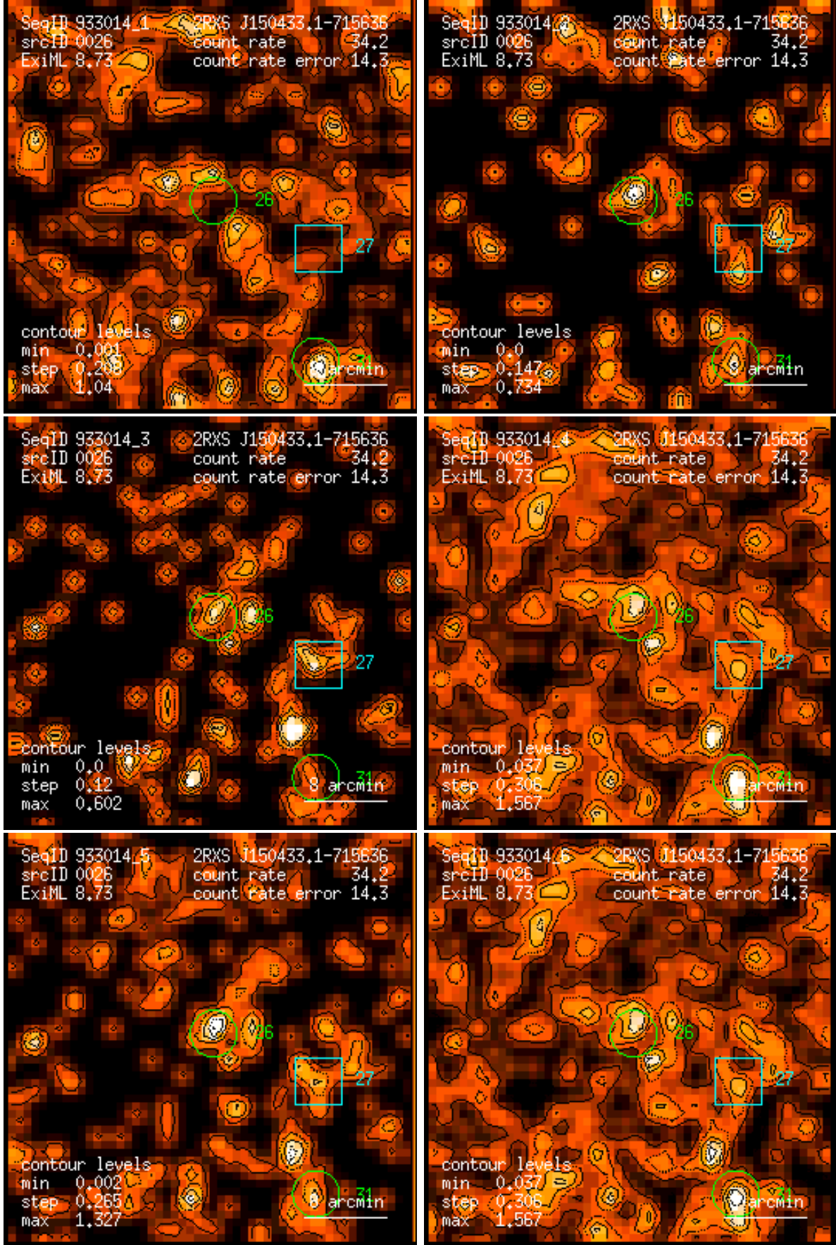
Figure 26: RASS 933014: detection 0026: band rate images, Gaussian filter: (1) PSPC channels 11 – 41, (2) 52 – 90, (3) 91 – 201, (4) 11 – 235, (5) 52 – 201, (6) 11 – 201. Broad band rates in counts/ks. Band rate contour levels in counts/ks/arcmin 2 .
