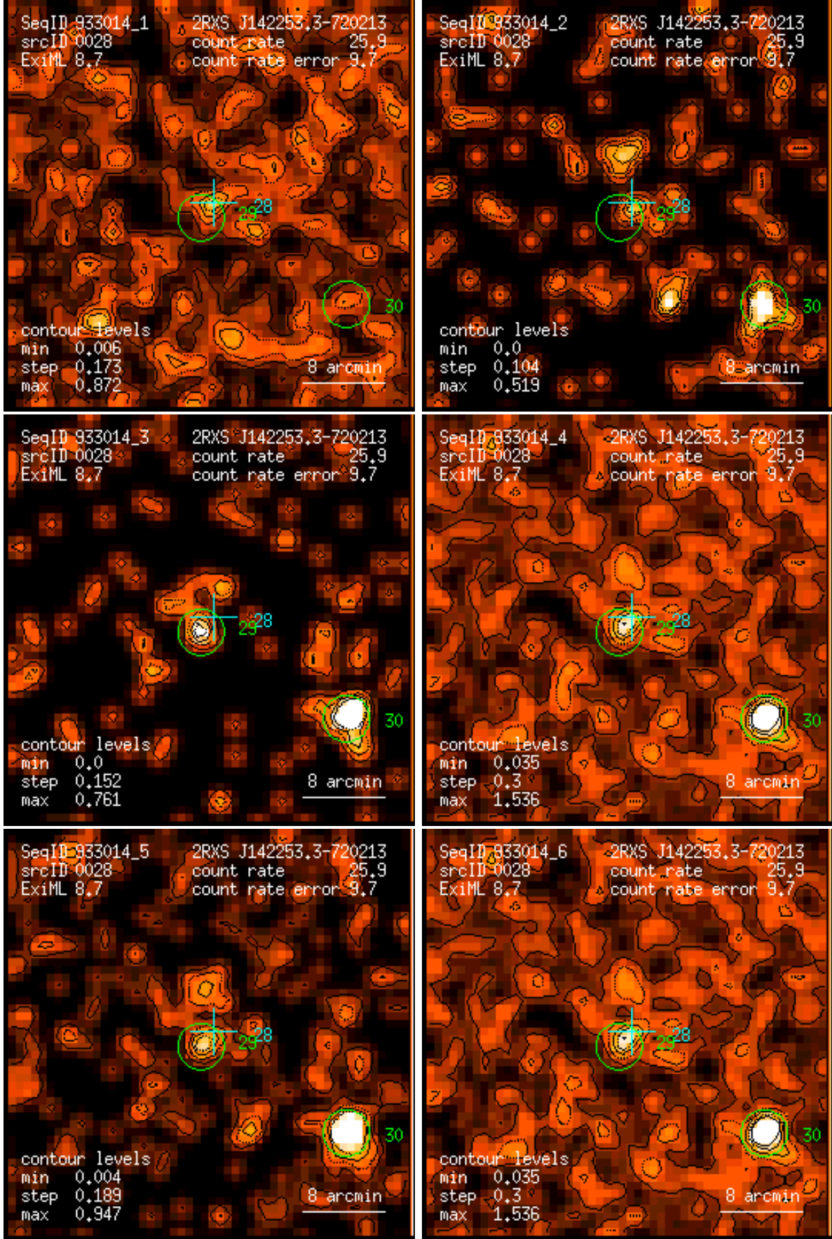
Figure 28: RASS 933014: detection 0028: band rate images, Gaussian filter: (1) PSPC channels 11 – 41, (2) 52 – 90, (3) 91 – 201, (4) 11 – 235, (5) 52 – 201, (6) 11 – 201. Broad band rates in counts/ks. Band rate contour levels in counts/ks/arcmin 2 .
