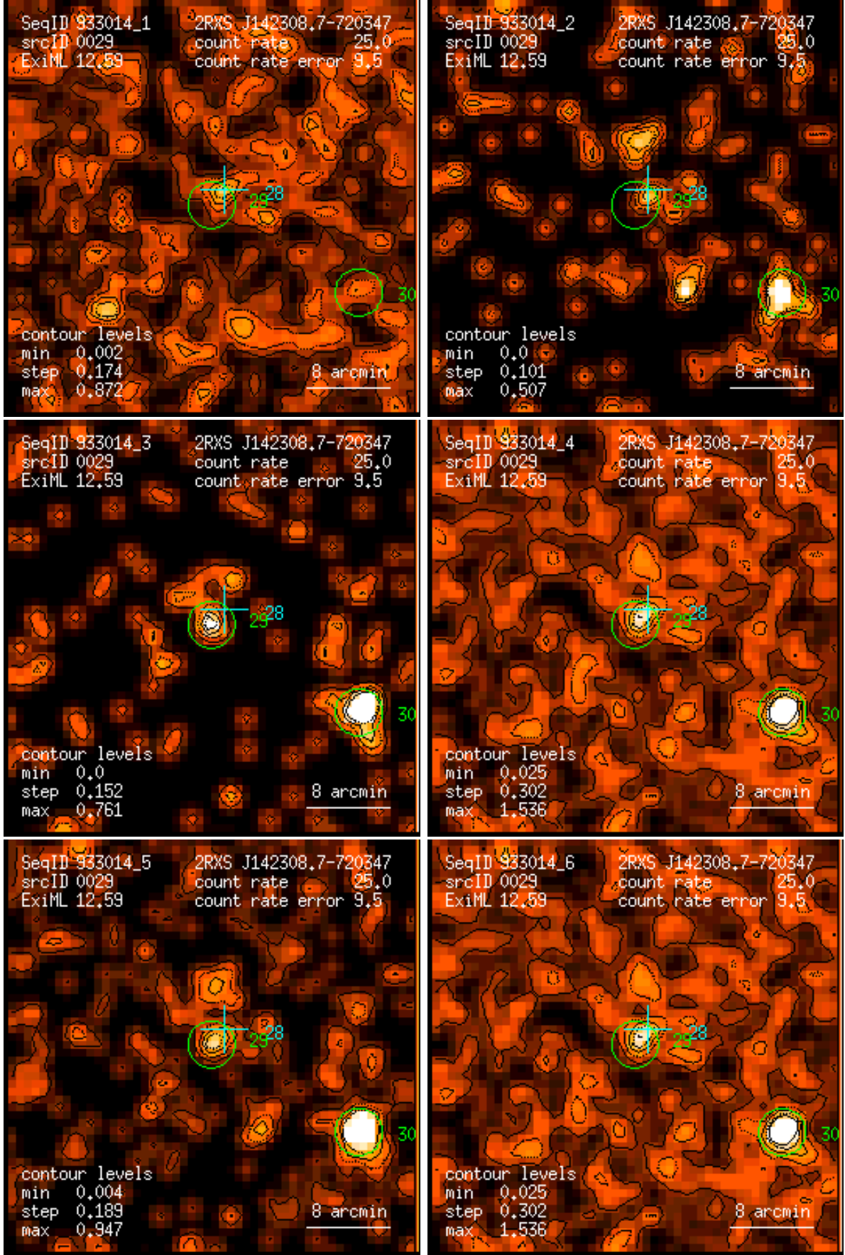
Figure 29: RASS 933014: detection 0029: band rate images, Gaussian filter: (1) PSPC channels 11 – 41, (2) 52 – 90, (3) 91 – 201, (4) 11 – 235, (5) 52 – 201, (6) 11 – 201. Broad band rates in counts/ks. Band rate contour levels in counts/ks/arcmin 2 .
