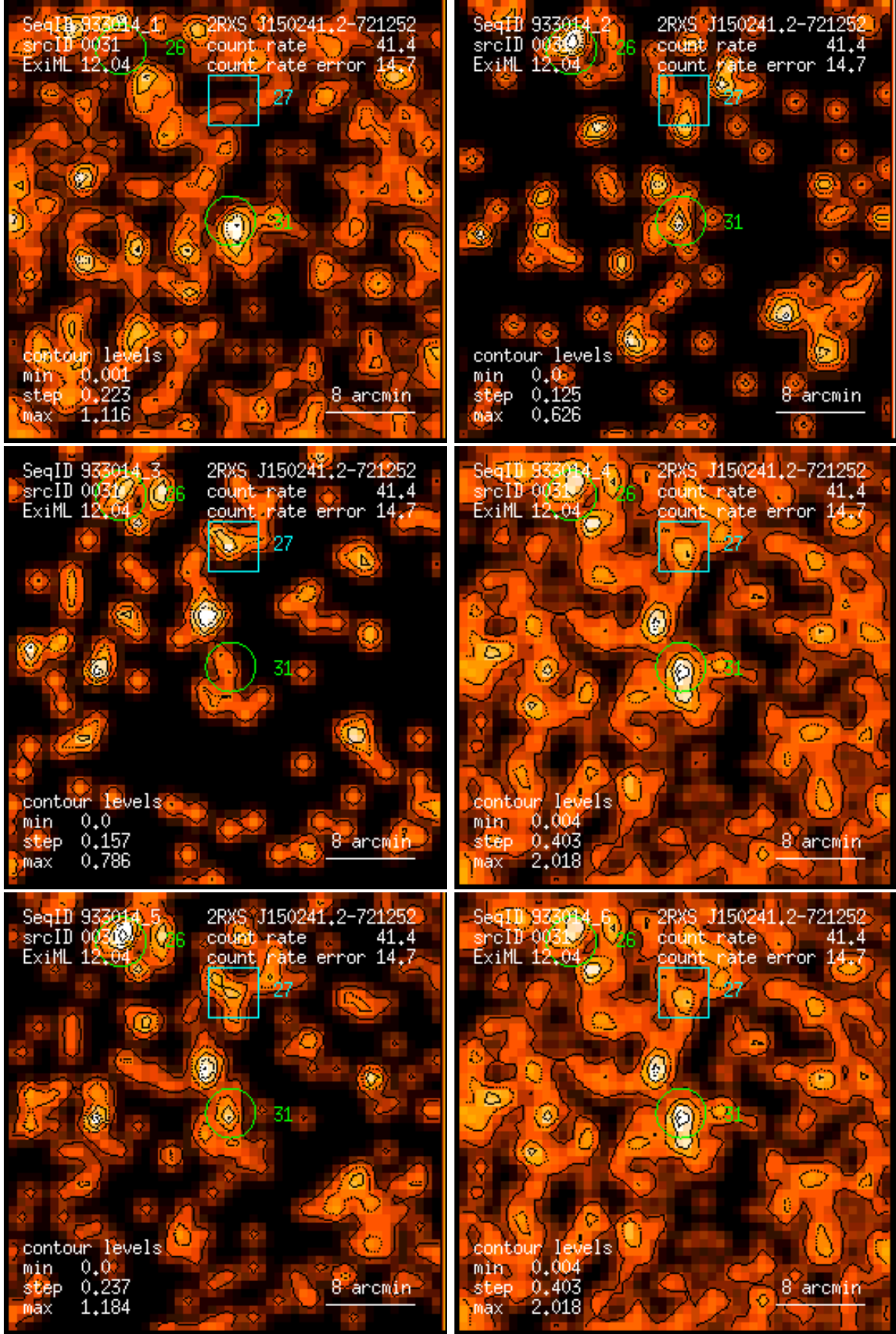
Figure 31: RASS 933014: detection 0031: band rate images, Gaussian filter: (1) PSPC channels 11 – 41, (2) 52 – 90, (3) 91 – 201, (4) 11 – 235, (5) 52 – 201, (6) 11 – 201. Broad band rates in counts/ks. Band rate contour levels in counts/ks/arcmin 2 .
