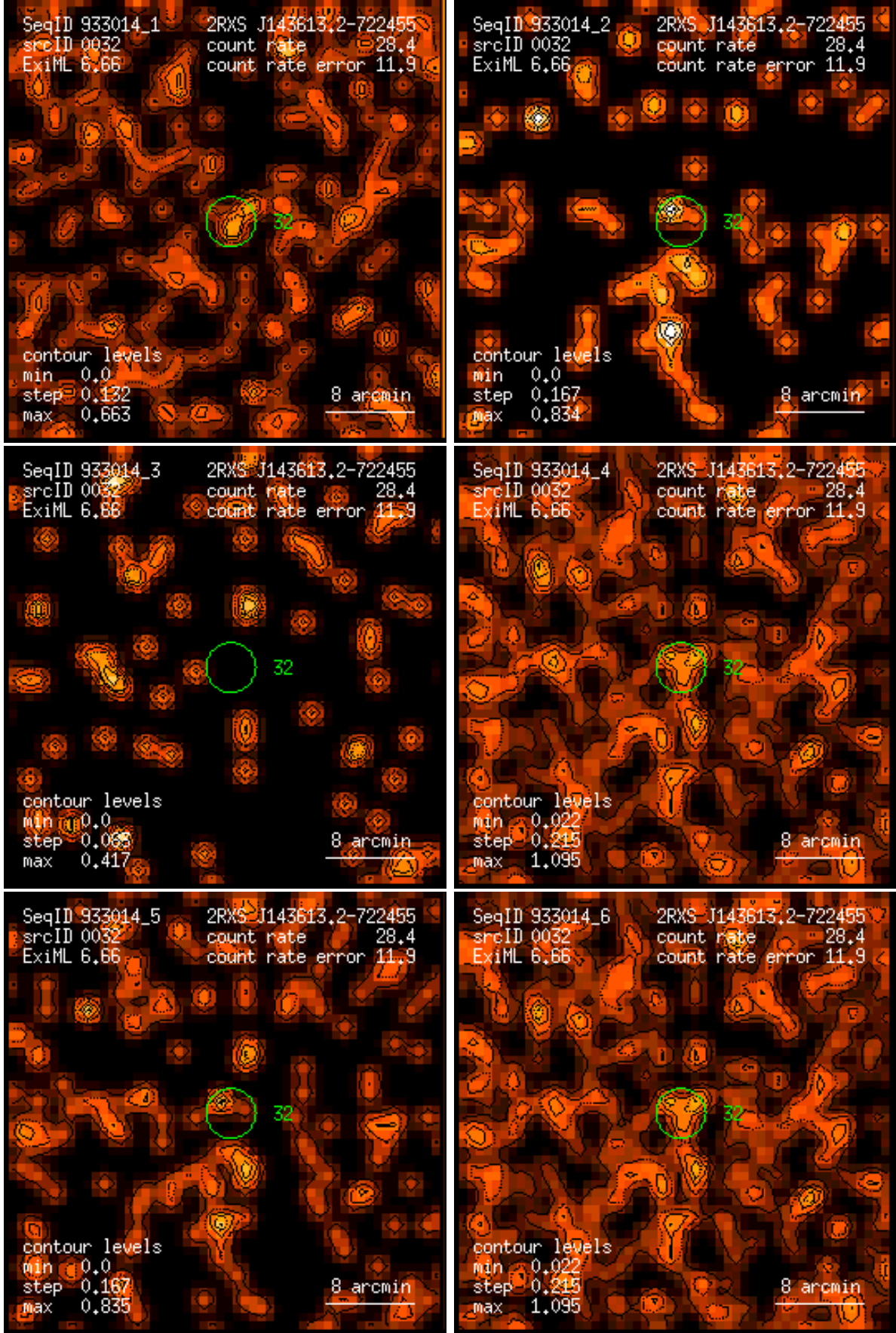
Figure 32: RASS 933014: detection 0032: band rate images, Gaussian filter: (1) PSPC channels 11 – 41, (2) 52 – 90, (3) 91 – 201, (4) 11 – 235, (5) 52 – 201, (6) 11 – 201. Broad band rates in counts/ks. Band rate contour levels in counts/ks/arcmin 2 .
